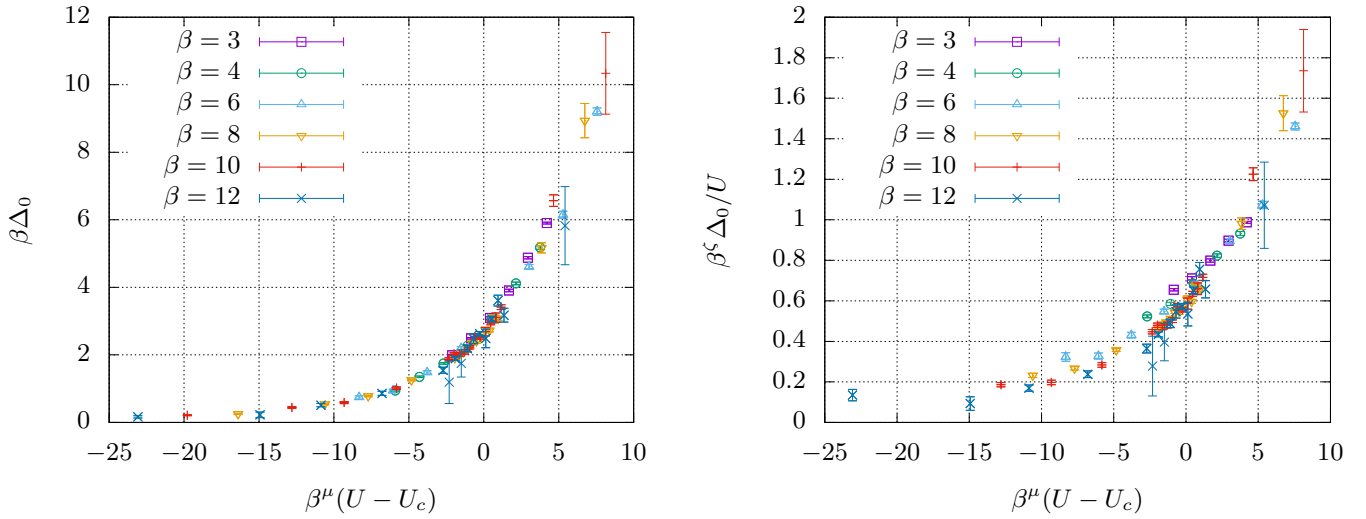
FIG. 4. f = \beta \Delta_0 (left) and g = \beta^\zeta \Delta_0 / U (right) as a function of u = \beta^\mu (U - U_c) according to Eqs. (31) and (33), respectively. All quantities are plotted with the parameters for optimal data collapse, and expressed in units of \kappa .
