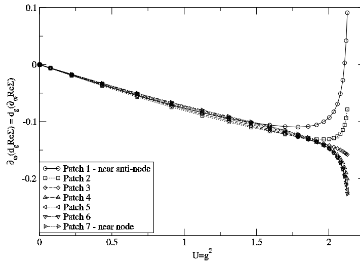
Figure 8: Flow of the "slope" of \frac{d}{dg} \text{Re}\Sigma on the Fermi surface from near anti-nodal (patch 1) to near nodal (patch 7) for T = 0.1 . The slope is defined as the Quasi-Fermi-liquid approximation, in analogy to Figure 2. The total number of discrete patches for this calculation was 728.
