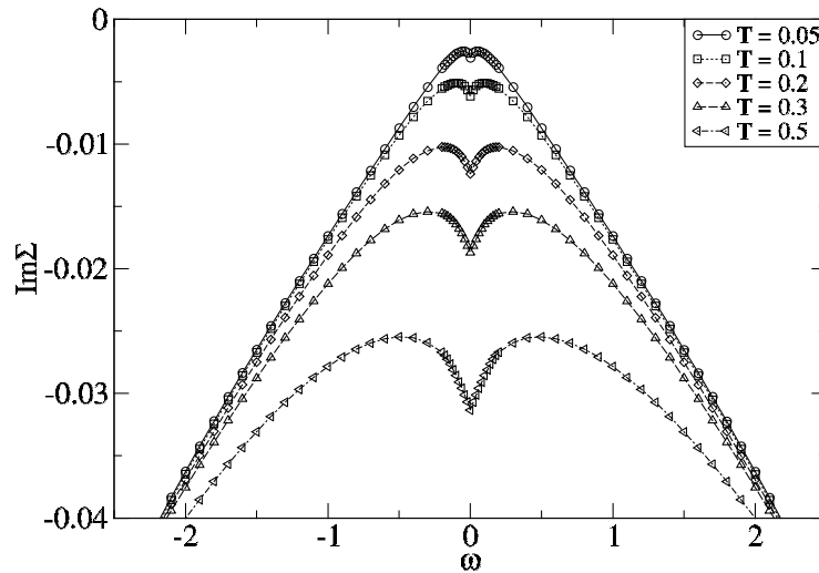
Figure 1: Raw data for Im\Sigma(\omega, \mathbf{k}_F) at U = 1.0 in second order bare perturbation theory. \mathbf{k}_F is chosen about half way between the nodal point (\pi/2, \pi/2) and the anti-nodal point (\pi, 0) . The down-turn at \omega = 0 increases with temperature and leads to a positive slope of Re\Sigma at \omega = 0 .
