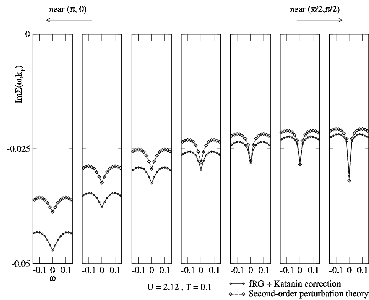
Figure 6: Self-energy corresponding to Figure 5
