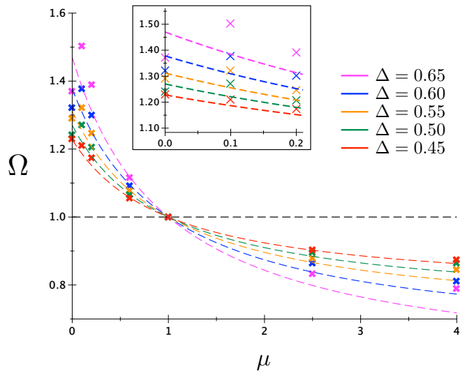
FIG. 2. Crosses: Rescaled ratio of velocities \Omega [see Eq. (11) for definition] obtained from PF simulations as a function of \mu , for different values of \Delta ; dashed colored lines: representation of Eq. (12) based on GF results for \mu = 0 and \mu = 1 ; black horizontal dashed line: Barbieri-Langer theory [19], i.e., Eq. (10).
