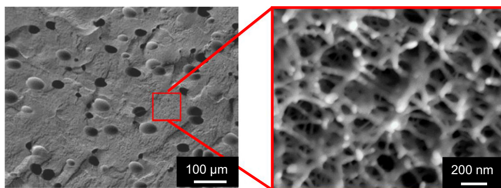
Fig. 7 SEM-images of the porous polystyrene obtained using the modified NF-CID method. A continuity-inversion of a close-packed PS nanoparticle assembly ( R_{\text{SEM}} = 23 \pm 3 \text{ nm} and a moderate polydispersity of p_{\text{SEM}} = 0.13 ) is induced due to a 30 min exposure to \text{CO}_2 at T = 65^\circ\text{C} , p = 250 \text{ bar} . After cooling the system down to T = 25^\circ\text{C} while keeping the pressure at p = 250 \text{ bar} , the pressure was slowly released. Gentle
