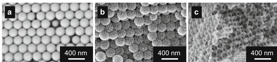
Fig. 8 SEM images of a) close-packed assemblies of monodisperse PS particles with a radius of R_{\text{SEM}} = 113 nm and p_{\text{SEM}} = 0.02 , b) close-packed assembly of monodisperse PS particles mineralized with ZnO after 5 deposition cycles, and c) ZnO inverse replica obtained after the annealing of b)
