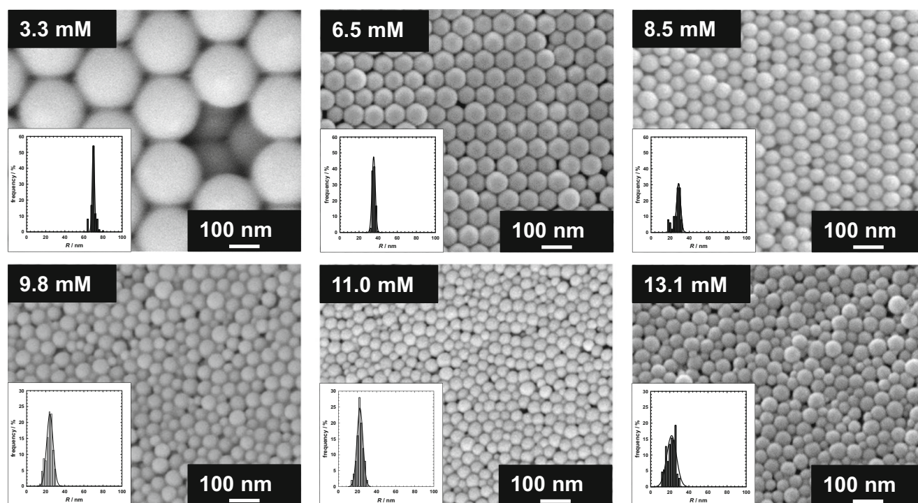
Fig. 4 Top view SEM images of close-packed PS nanoparticles as well as particle size distribution (inset), synthesized at various [SDS] and at T = 80^\circ\text{C} . Increasing [SDS] to > 8.5\text{ mM} the ordering of the particle
