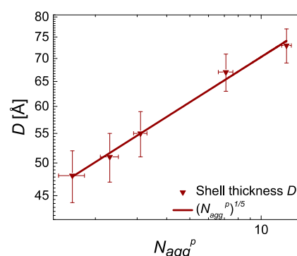
Figure 4. Halperin plot of shell thickness D versus aggregation number of the polymer N_{agg}^p for each measured mixture of C_{28} -PEO5 and SDS at various concentrations.
