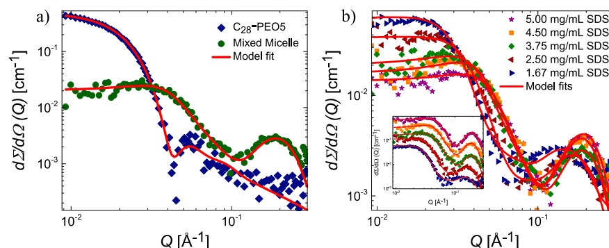
Figure 3. (a) SAXS scattering curves of 5.00 mg/mL C_{28} -PEO5 with core-shell model fit, and equilibrated mixture of 5.00 mg/mL C_{28} -PEO5 + 3.75 mg/mL SDS, fitted with the new MM model. (b) SAXS scattering curves of equilibrated 5.00 mg/mL C_{28} -PEO5 mixed with various concentrations of SDS. A clear trend toward smaller micelles with larger SDS concentration can be seen. The inset in (b) provides scaled scattering data to show the shift to higher Q values with higher concentrations of SDS.
