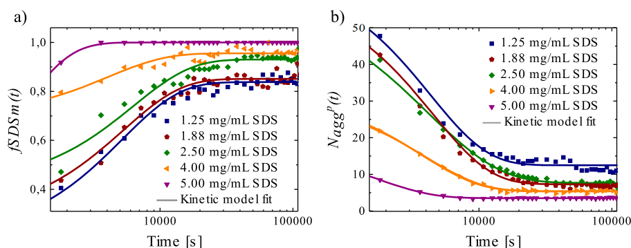
Figure 9. Evolution of the structural parameters on a logarithmic time scale where the molar ratio SDS/C 28 -PEOS was held constant at 9.3. The concentration of C 28 -PEOS is the double of the given concentrations of SDS. (a) Fraction of SDS in the mixed micelles ( f_{SDSm}(t) ) and (b) aggregation number of polymer ( N_{agg}^p(t) ) over time, fitted with the kinetic model.
