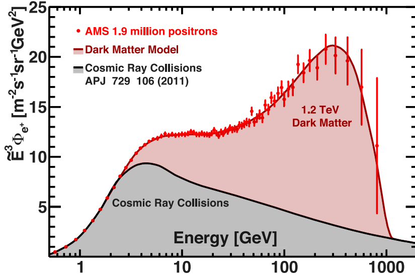
Fig. 43. Comparison of the AMS data (red data points) with predictions of a dark matter model based on Ref. [62] with M_\chi = 1.2\text{ TeV} (brown curve and shading). Also shown is a model prediction of cosmic ray collisions [72] (black curve and shading).
