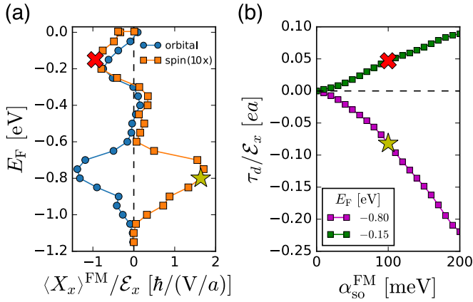
FIG. 4. (a) \langle S_x \rangle^{\text{FM}} / \mathcal{E}_x (orange squares for 10\times magnified values) as a function of E_F with \alpha_{\text{so}}^{\text{FM}} = 100 meV. For comparison, \langle L_x \rangle^{\text{FM}} / \mathcal{E}_x (blue circles) is also shown. (b) \tau_d / \mathcal{E}_x as a function of \alpha_{\text{so}}^{\text{FM}} with E_F = -0.80 eV (purple squares) and E_F = -0.15 eV (green squares). The yellow star and red cross symbols in (a) and (b) are obtained for the same E_F and \alpha_{\text{so}}^{\text{FM}} . For this calculation, smaller system size is used ( N_{\text{NM}} = 8 and N_{\text{FM}} = 2 ).
