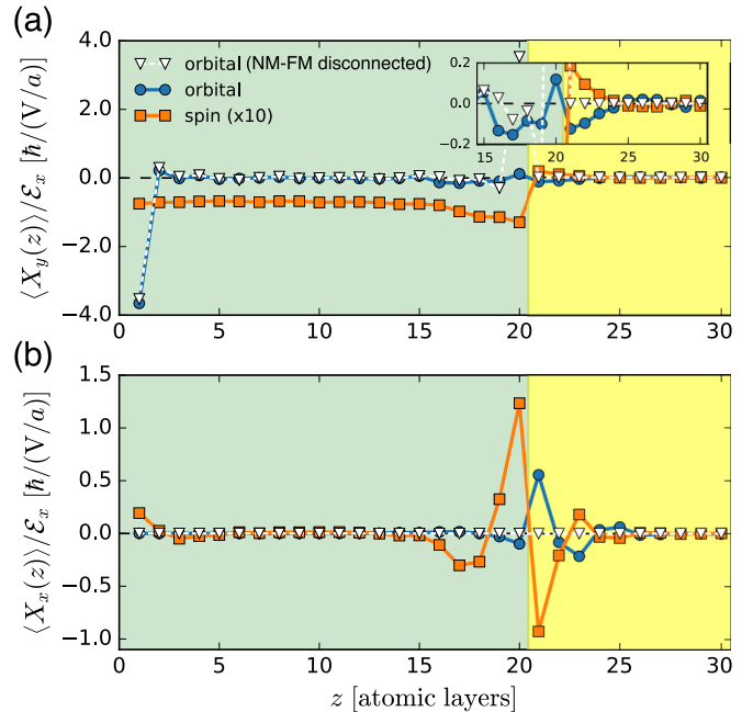
FIG. 5. (a) \langle X_y(z) \rangle / E_x and (b) \langle X_x(z) \rangle / E_x as a function of z for E_F = -0.9 eV, when the relative sign of the interface hoppings is flipped [Eq. (B1)]. Blue circles (orange squares) depict the orbital (spin multiplied by factor 10) accumulation profile in the NM ( 1 \leq z \leq 20 ) and the FM ( 21 \leq z \leq 30 ). White inverted triangles depict the orbital accumulation profile when the NM and FM are disconnected. The inset in (a) presents a magnified plot near the NM/FM interface.
