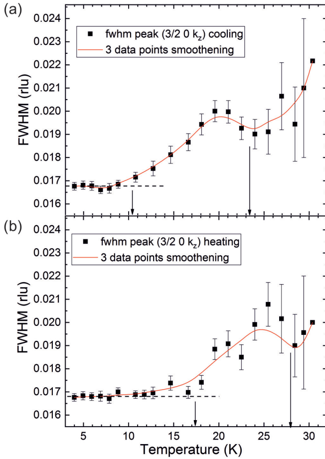
FIG. 4. Temperature dependence of the FWHM for the magnetic Bragg reflection (200)^{-k_2} as obtained from the fit with one Gaussian peak, (a) by cooling and (b) by heating. Data points are presented by the black squares; the red lines are the smoothing function by three neighboring points applied to the data as a guide for the eyes. The black arrows indicate the temperature region where an “intermediate” magnetic phase with k_{z2} is supposed to exist (see main text for more details).
