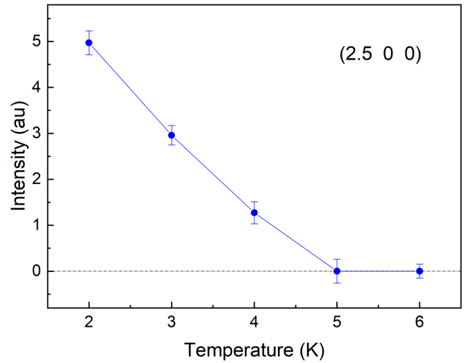
FIG. 5. Temperature dependence of the magnetic Bragg reflection (200)^{+k_{Nd}} by heating with commensurate propagation vector k_{Nd} = (1/2 0 0) , associated with spontaneous ordering of the Nd^{3+} magnetic sublattice.
