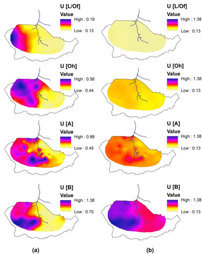
Figure 3. Spatial distribution of U in the catchment area for the four principal soil horizons (L/Of, Oh, A, and B, top to bottom rows) using ordinary kriging, represented using (a) different color bars, and (b) one color bar for all horizons. Notice the individual legend for each horizon for U (mg kg -1 ) concentration distributions. Extreme outliers were identified in R (Version 3.3.2, R Core Team, Vienna, Austria) by setting the upper and lower limits as the quartile (lower or upper) plus or minus three times the inter quartile range.
