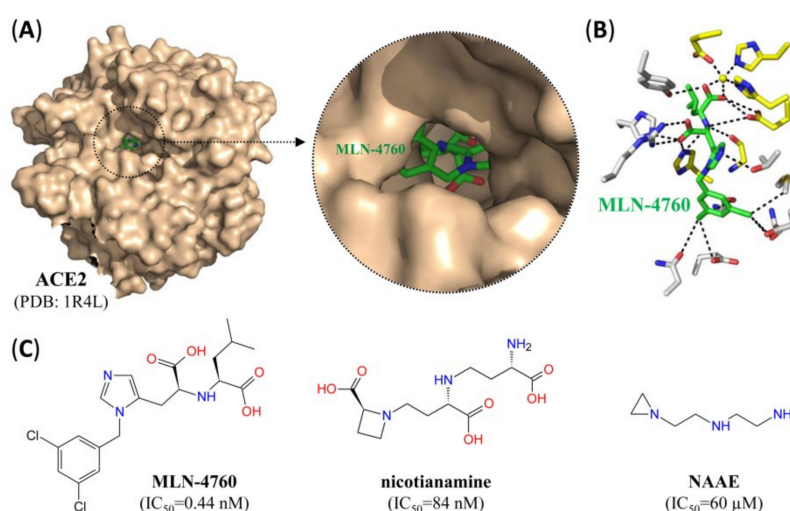
Figure 3. Mechanism of action and structure of small molecule ACE2 inhibitors. (A) Surface representation of the crystal structure of ACE2 with the small molecule inhibitor MLN-4760 (green) bound to the active site. Inset: close-up view showing part of the inhibitor bound to the active site. (B) Stick representation of MLN-4760 (green) bound to residues at the active site. Catalytic residues and the active site zinc ion are indicated in yellow. Dashed black lines indicate formation of hydrogen bonds. (C) Structure of different small molecule inhibitors of ACE2 and IC_{50} values for suppression of human ACE2.
