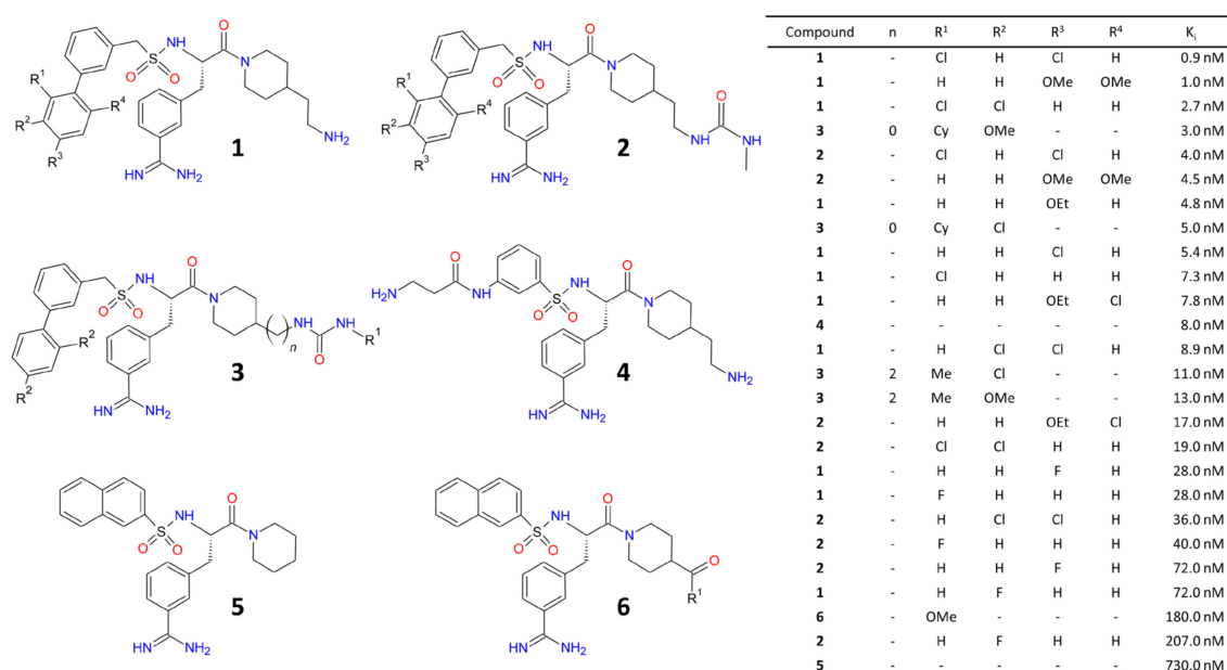
Figure 4. Structure–activity relationship of small molecule TMPRSS2 inhibitors. Shown are various synthetic inhibitors with sulfonlated 3-amindinophenylalanilamide moieties. For details and additional structures, see [42].
