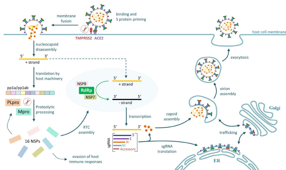
Figure 2. SARS-CoV-2 replication and transcription cycle in infected cells. Schematic representation of the processes involved in the replication of SARS-CoV-2 in infected host cells. For details see Sections 2.2 and 2.3.
