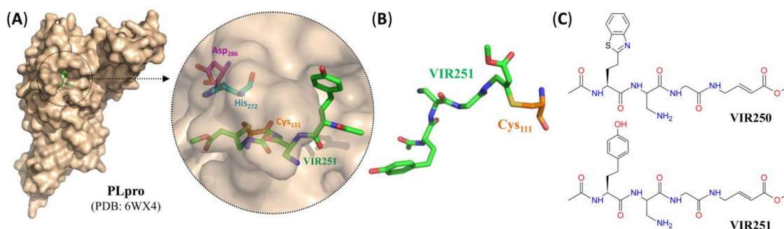
Figure 9. SARS-CoV-2 PLpro peptidomimetic inhibitors with an electrophilic vinyl methyl ester warhead. (A) Surface representation of the crystal structure of PLpro from SARS-CoV-2 with VIR251 (green) bound to the active site. Inset: close-up view of the inhibitor-bound active site, with residues forming the catalytic triad indicated in turquoise (His 272 ), orange (Cys 111 ) or purple (Asp 286 ) and hydrogen bonds indicated by dashed black lines. (B) Stick representation of VIR251 (green) covalently bound to the catalytic cysteine residue (orange). (C) Structure of different peptidomimetic SARS-CoV-2 PLpro inhibitors with electrophilic vinyl methyl ester warhead. For pharmacological properties, see Table 3.
