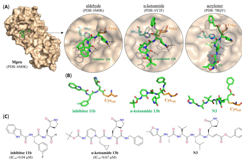
Figure 5. SARS-CoV-2 Mpro peptidomimetic inhibitors with different electrophilic warheads. (A) Surface representation of one protomer from the crystal structure of SARS-CoV-2 Mpro with the peptidomimetic inhibitor 11b (green) bound to the active site. Insets: close-up view of the active site after covalent modification by (from left to right) inhibitor 11b with an aldehyde warhead, \alpha -ketoamide 13b with an \alpha -ketoamide warhead or N3 with an acrylate warhead (green). Residues forming the catalytic dyad are indicated in turquoise (His 41 ) or orange (Cys 145 ) and hydrogen bonds are indicated by dashed black lines. (B) Stick representations of (from left to right) aldehyde inhibitor 11b, \alpha -ketoamide 13b and acrylate N3 (green) covalently bound to the catalytic cysteine residue (orange). (C) Structure of (from left to right) aldehyde inhibitor 11b, \alpha -ketoamide 13b and acrylate N3. For pharmacological properties see Table 2. For the structures of additional peptidomimetic inhibitors with aldehyde or \alpha -ketoamide warheads listed in Table 2, see Appendix A at the end of the article.
