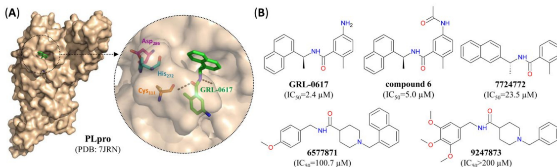
Figure 8. SARS-CoV-2 PLpro small molecule non-covalent inhibitors. (A) Surface representation of the crystal structure of PLpro from SARS-CoV-2 with GRL-0617 (green) bound to the active site. Inset: close-up view of the inhibitor-bound active site, with residues forming the catalytic triad indicated in turquoise (His 272 ), orange (Cys 111 ) or purple (Asp 286 ) and hydrogen bonds indicated by dashed black lines. (B) Structure of different small molecule non-covalent SARS-CoV-2 PLpro inhibitors. For pharmacological properties, see Table 3.
