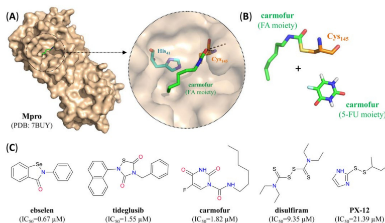
Figure 6. SARS-CoV-2 Mpro small molecule covalent inhibitors. (A) Surface representation of one protomer from the crystal structure of SARS-CoV-2 Mpro with the carmofur fatty acid moiety (green) bound to the active site. Inset: close-up view of the inhibitor-bound active site, with residues forming the catalytic dyad indicated in turquoise (His 41 ) or orange (Cys 145 ) and hydrogen bonds indicated by dashed black lines. (B) Stick representation of the fatty acid (FA) moiety of carmofur (green) covalently bound to the catalytic cysteine residue (orange). In addition, the 5-fluorouracil (5-FU) moiety released during binding of carmofur to the active site is also shown. (C) Structure of different small molecule covalent SARS-CoV-2 Mpro inhibitors. For pharmacological properties, see Table 2.
