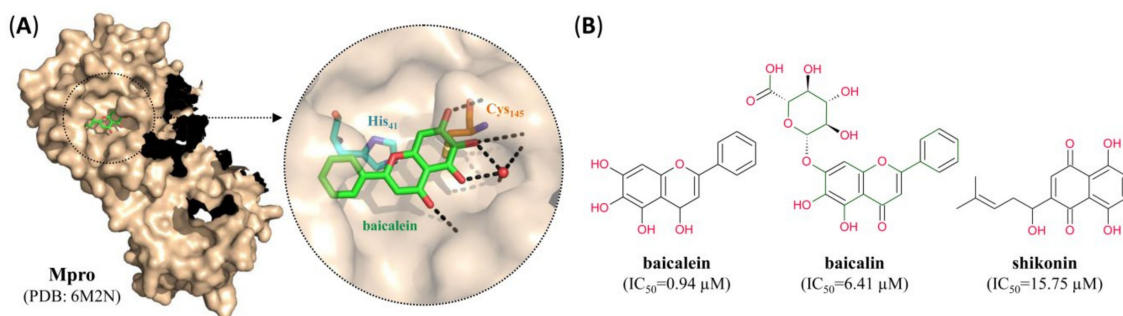
Figure 7. SARS-CoV-2 Mpro small molecule non-covalent inhibitors. (A) Surface representation of one protomer from the crystal structure of SARS-CoV-2 Mpro with baicalein (green) bound to the active site. Inset: close-up view of the inhibitor-bound active site, with residues forming the catalytic dyad indicated in turquoise (His 41 ) or orange (Cys 145 ) and hydrogen bonds indicated by dashed black lines. (B) Structure of different small molecule non-covalent SARS-CoV-2 Mpro inhibitors. For pharmacological properties, see Table 2.
