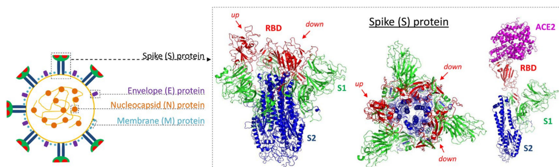
Figure 1. Structure of severe acute respiratory syndrome coronavirus 2 (SARS-CoV-2). Schematic representation illustrating the 4 structural proteins of SARS-CoV-2. Inset shows side (left) and top (middle) view of homotrimeric spike glycoprotein with two of the receptor binding domains (RBD, red) in their down position and one in the up position. The rightmost structure shows a single monomer with the RBD in its up position and bound to human ACE2. Protein structures visualized with PyMol using models from https://swissmodel.expasy.org .
