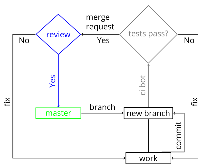
FIG. 6. Continuous integration workflow integrated with git.
