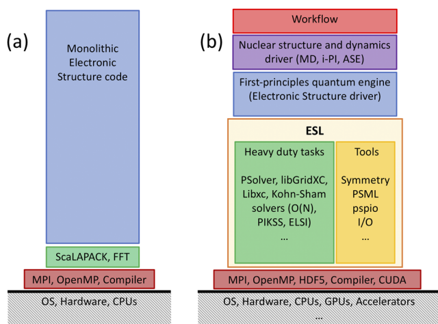
FIG. 1. Comparison of the traditional monolithic and emerging modular paradigms in electronic structure coding. One of today's electronic-structure codes—large blue box in panel (a)—thins down into the higher-level electronic structure driver that defines the particular code—blue box in panel (b), allowing for a more specialized and sustainable development of the different parts of the software. The acronyms indicate operating system (OS), fast Fourier transforms (FFT), input/output (I/O), molecular dynamics (MD), and linear scaling with the number of atoms, O(N) , in addition to the central and graphical processing units, CPU and GPU, respectively. Steering upper-level drivers are distinguished between versatile toolkits, such as ASE, and handlers of massive amounts of quantum-engine replicas, such as i-PI. In addition to the well-known MPI, OpenMP, CUDA, and HDF libraries, other acronyms and names related to libraries are described in Secs. I, II, and IV.
