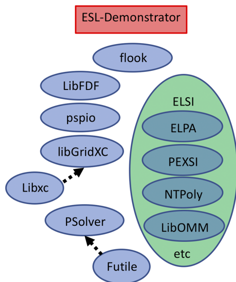
FIG. 5. Libraries used in the full DFT program developed as a demonstrator for the ESL. It allows the user to choose between plane-waves and atomic orbitals as basis sets. The libraries themselves are as in Fig. 4, and as described in this section.
