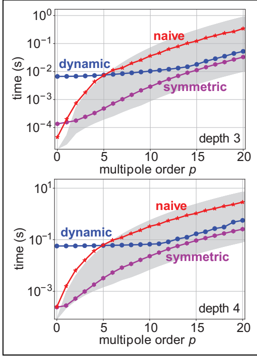
Figure 16. Runtime comparison of the three different M2L implementations. For each multipole order, 8^D \times 189 single M2L operations are computed for D = 3 (top) and D = 4 (bottom). The gray area marks the gap between the memory bound and the compute-bound reference microkernel shown in Figure 15.
