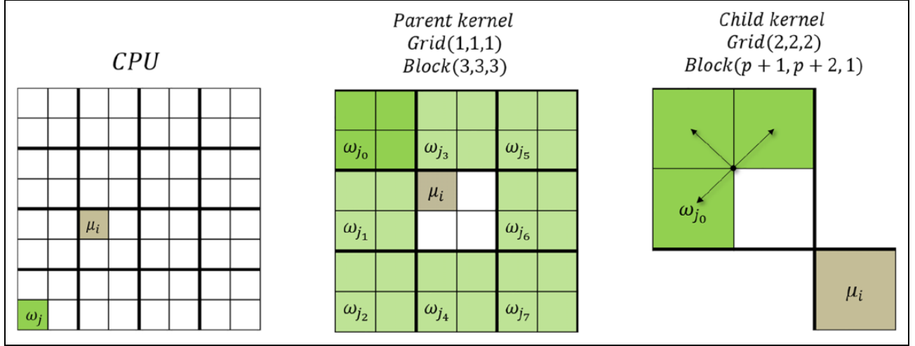
Figure 7. Dynamic M2L scheme. The CPU computes a \mu_i^d and the corresponding \mathcal{L}_i^d . The parent kernel determines all valid \mathcal{P}_j^d \subseteq \mathcal{L}_i^d sets, whereas the child kernel performs the M2L operations for \omega_{j_k}^d, j_k \in \mathcal{P}_j^d, k = 0, \dots, 7 and the target \mu_i^d .
