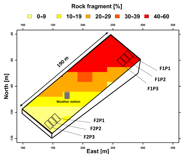
Figure 1. Description of the location of field experiment and setup of water treatments in the stony soil (F1) and silty soil (F2). P1–P3 are the sheltered, rainfed, and irrigated plots. Rock fragments are gravels with weathered granites.
