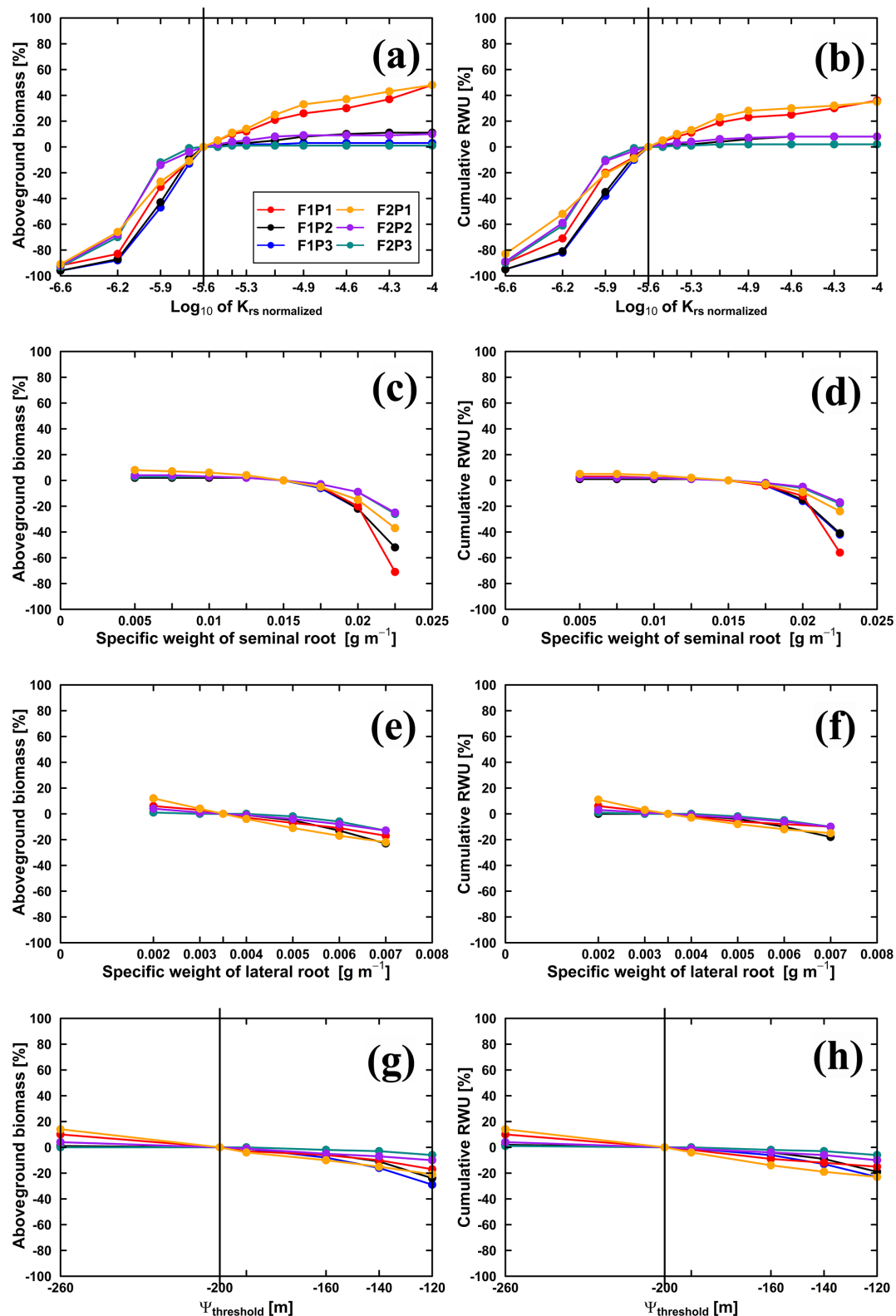
Figure 11. Relative changes of simulated (Co model) aboveground biomass at harvest (a, c, e, g) and cumulative RWU (b, d, f, h) (from 15 March to harvest on 23 July 2016) with the changing K_{rs, \text{normalized}} , specific weights of seminal and lateral roots and leaf pressure head threshold ( \Psi_{\text{threshold}} ) in the sheltered (P1), rainfed (P2), and irrigated (P3) plots of the stony soil (F1) and the silty soil (F2). Vertical lines in (a, b) indicate the original value K_{rs, \text{normalized}} = 0.2554 \times 10^{-5} \text{ cm d}^{-1} , while in (g, h) the vertical lines indicate the \Psi_{\text{threshold}} = -200 \text{ m} .
