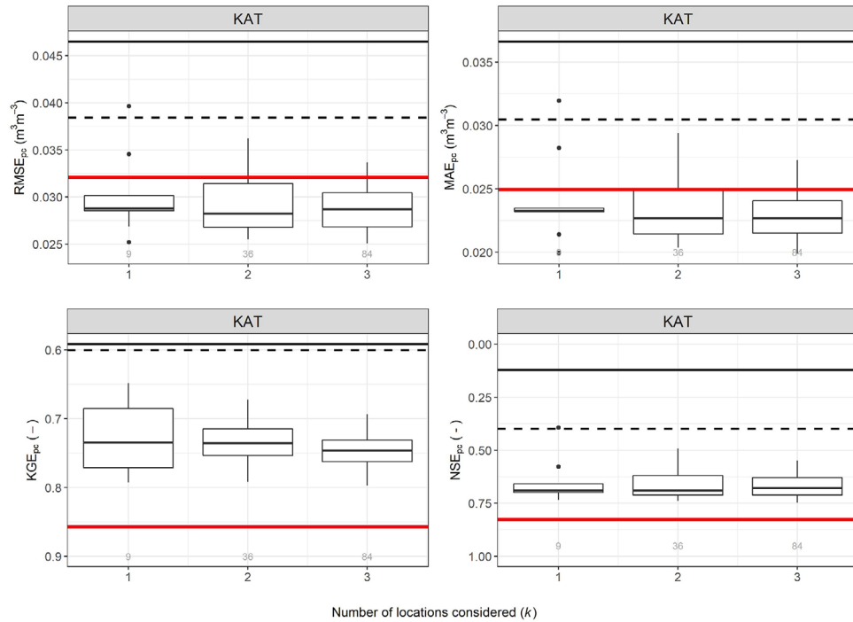
FIGURE D4 Comparison of the analysis for the performance measures for depth d = 50 , radial distance r = 75 , and sample size k = 1, 2 , and 3 at the field site Katharinentaler Hof (KAT). Panels show the profile shape correction performance for root mean square error, mean absolute error, Kling–Gupta efficiency, and Nash–Sutcliffe efficiency (RMSE pc , MAE pc , KGE pc , and NSE pc ). Baseline performance for each measure is marked as a black line, the reference performance is marked as a red line, and the bias performance is marked with a black and dashed line. The RMSE pc is the same as presented in Figure 6.
