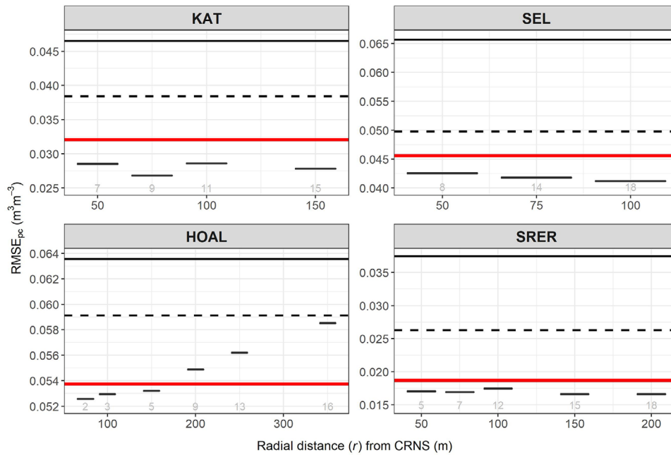
FIGURE 5 RMSE_{pc} (profile shape correction performance using the root mean square error [RMSE]) considering different radial distances of the point soil moisture locations from the cosmic-ray neutron sensor (CRNS). With increasing radii, the number of available locations used for the profile shape correction increases (gray numbers below boxes). The red line marks the RMSE_{ref} (reference performance), and the black line marks the RMSE_{base} (baseline performance), and the dashed line marks the RMSE_{bias} (bias performance). HOAL, Hydrological Open Air Laboratory; KAT, Katharinentaler Hof; SEL, Selhausen; SRER, Santa Rita Experimental Range
