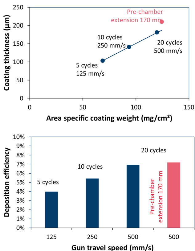
Fig. 4 Area-specific coating weights and deposition efficiencies for different combinations of gun travel speeds and number of spray passes; in addition, a prechamber extension of 170 mm was tested with the last parameter set
