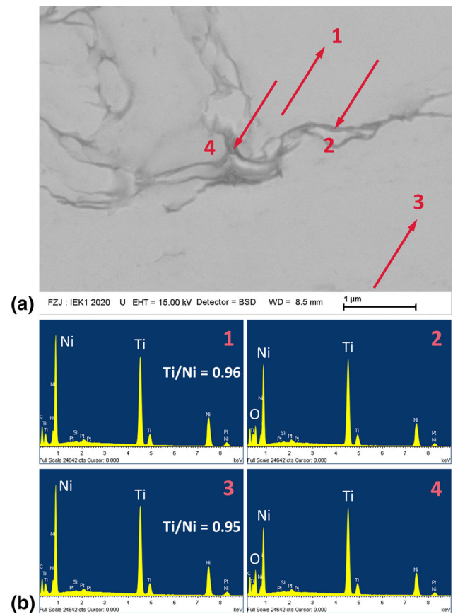
Fig. 8 EDS point analyses of a NiTi coating sprayed in 5 passes with 125 mm/s gun travel speed; (a) backscattered electron image with EDS positions 1-4 indicated by arrows; (b) energy spectra 1-4 with highlighted Ni, Ti and O peaks; the quantitative Ti/Ni atomic ratios could not be given reliably for the oxide films (spectra 2 and 4) due to their small thicknesses compared to the dimensions of the material volume excited by the electron beam
