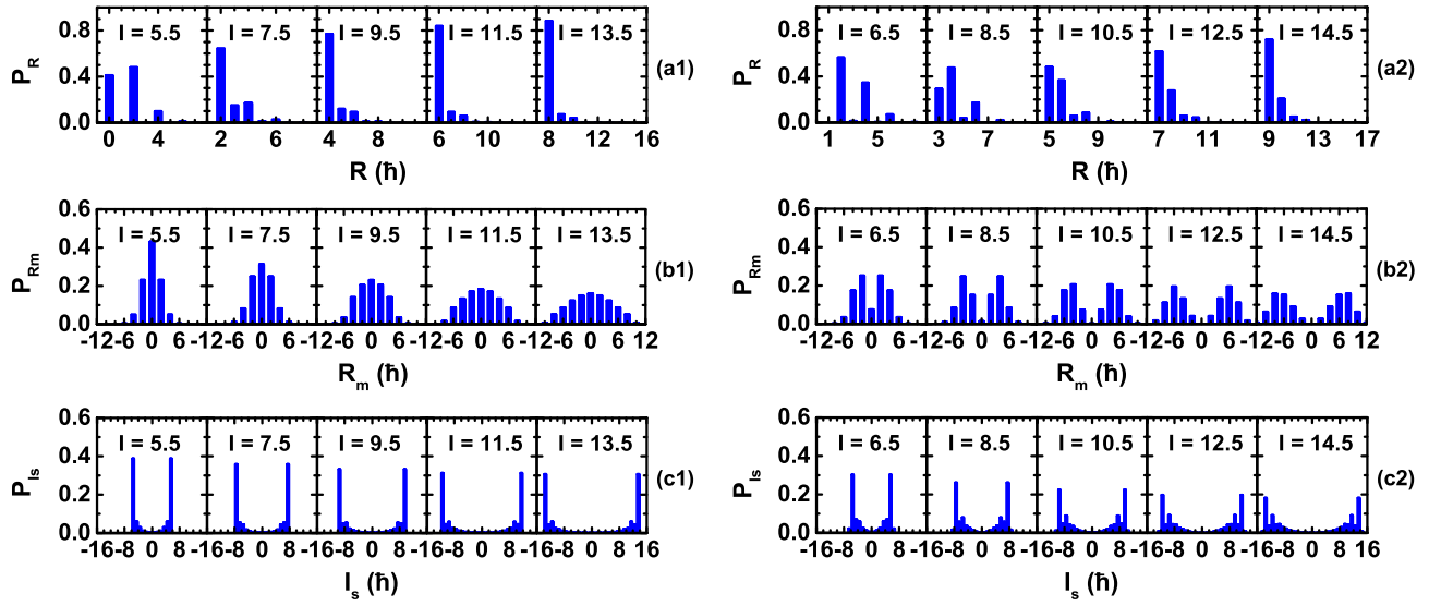
Fig. 4. Probability distributions for the rotor angular momentum ( R -plot P_R , a1-a2), for the projection of the rotor angular momentum onto the m -axis ( K_R -plot P_{Rm} , b1-b2), and for the projection of the total angular momentum onto the s -axis ( K -plot P_{Is} , c1-c2) as calculated in the PRM for states in the yrast and wobbling bands of ^{133}\text{La} .
