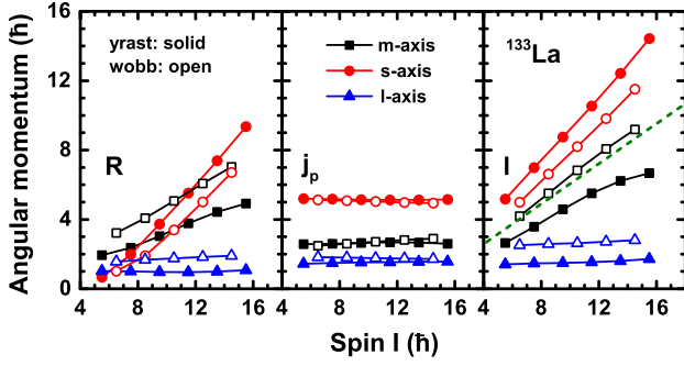
Fig. 2. Angular momentum components along the intermediate ( m -), short ( s -), and long ( l -) axis of the rotor, proton-particle, and total nuclear system as functions of the spin I for the yrast and wobbling bands in ^{133}\text{La} . Each component is a root-mean-square expectation value of an angular momentum operator, e.g. I_s = \langle \hat{I}_s^2 \rangle^{1/2} . The dashed lines correspond to the average quantity \sqrt{I(I+1)/3} .
