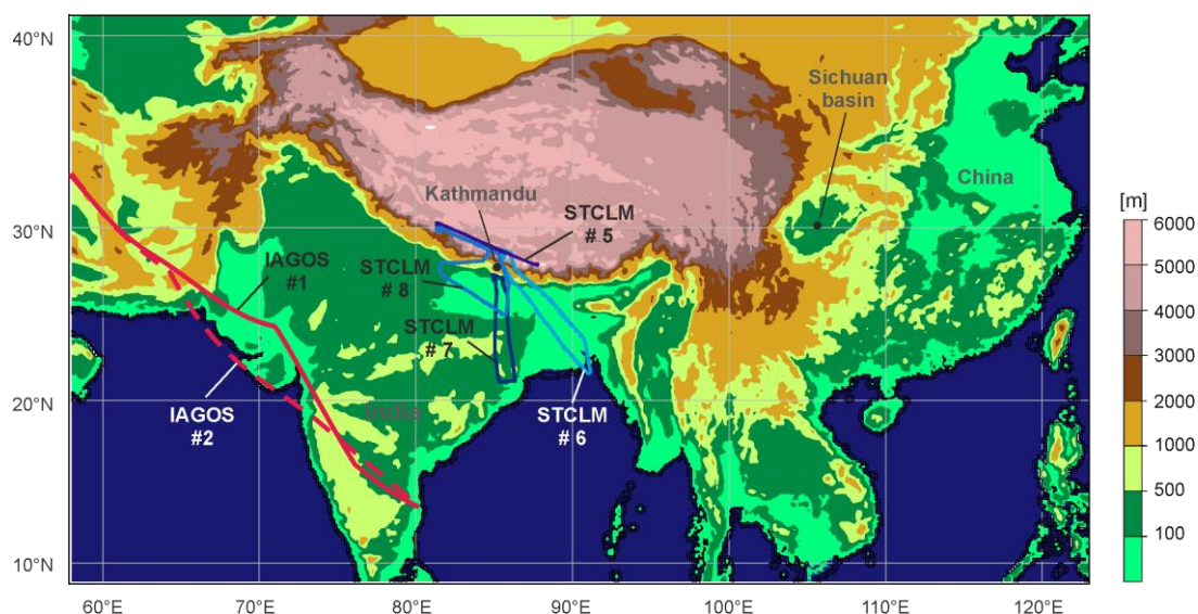
Figure 1. Topography and domain considered in the Meso-NH numerical simulation with a resolution of 15 km. The trajectory of the 675 Geophysica flights #5, #6, #7, and #8 during the StratoClim campaigns (marked with ‘STCLM’) around and south of Kathmandu are shown by the bluish solid lines, while two IAGOS flight tracks (to/from Madras in India) are indicated by the red solid and dashed line.
