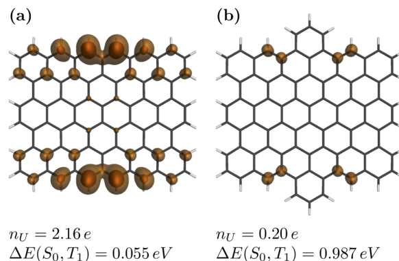
FIG. 4. MRCI computations on two different graphene nanoflakes: (a) a periacene with an unperturbed zig-zag edge and (b) the same system with two additional phenyl rings. The contour plots represent the distribution of unpaired electrons (isovalues of 0.005/0.0005 \text{ a.u.} ).
