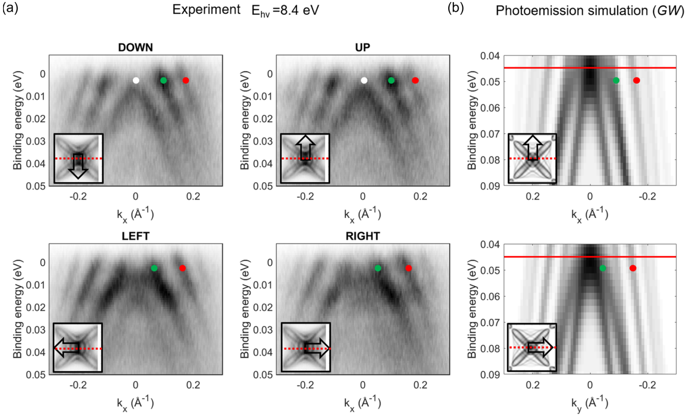
FIG. 8. (a) Experimental result obtained using unpolarized light of E_{h\nu} = 8.4 eV for a 40-ML-thick sample remanently magnetized along different in-plane directions. (b) Results of the corresponding photoemission simulations. Insets clarify the orientation of the cuts in k space (red dotted line) with respect to the magnetization direction (arrow). Red horizontal lines in (b) indicate position of the experimental Fermi level. Colored dots mark corresponding QWS.
