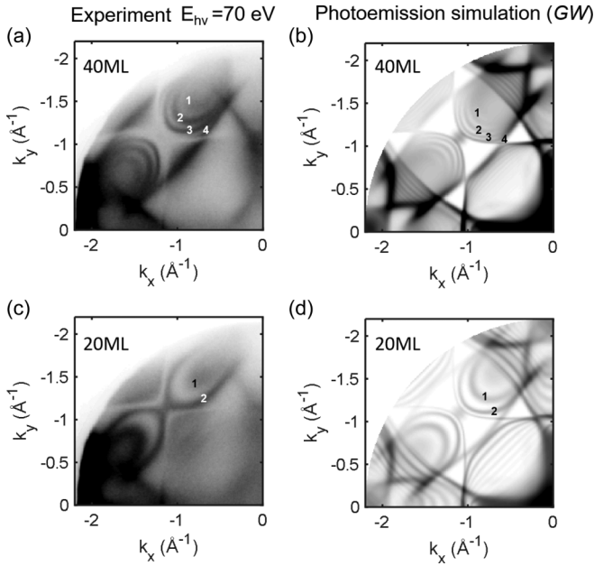
FIG. 5. Quantum well states near the Fermi level ( E_b = 0.05 eV). Comparison of the photoemission intensities obtained using p -polarized light of E_{hv} = 70 eV for 40-ML-thick sample (a) and 20-ML-thick sample (c). The magnetization direction and the photon incidence direction are the same as in Fig. 4. (b, d) Corresponding photoemission simulations. The numerals mark corresponding quantum well states.
