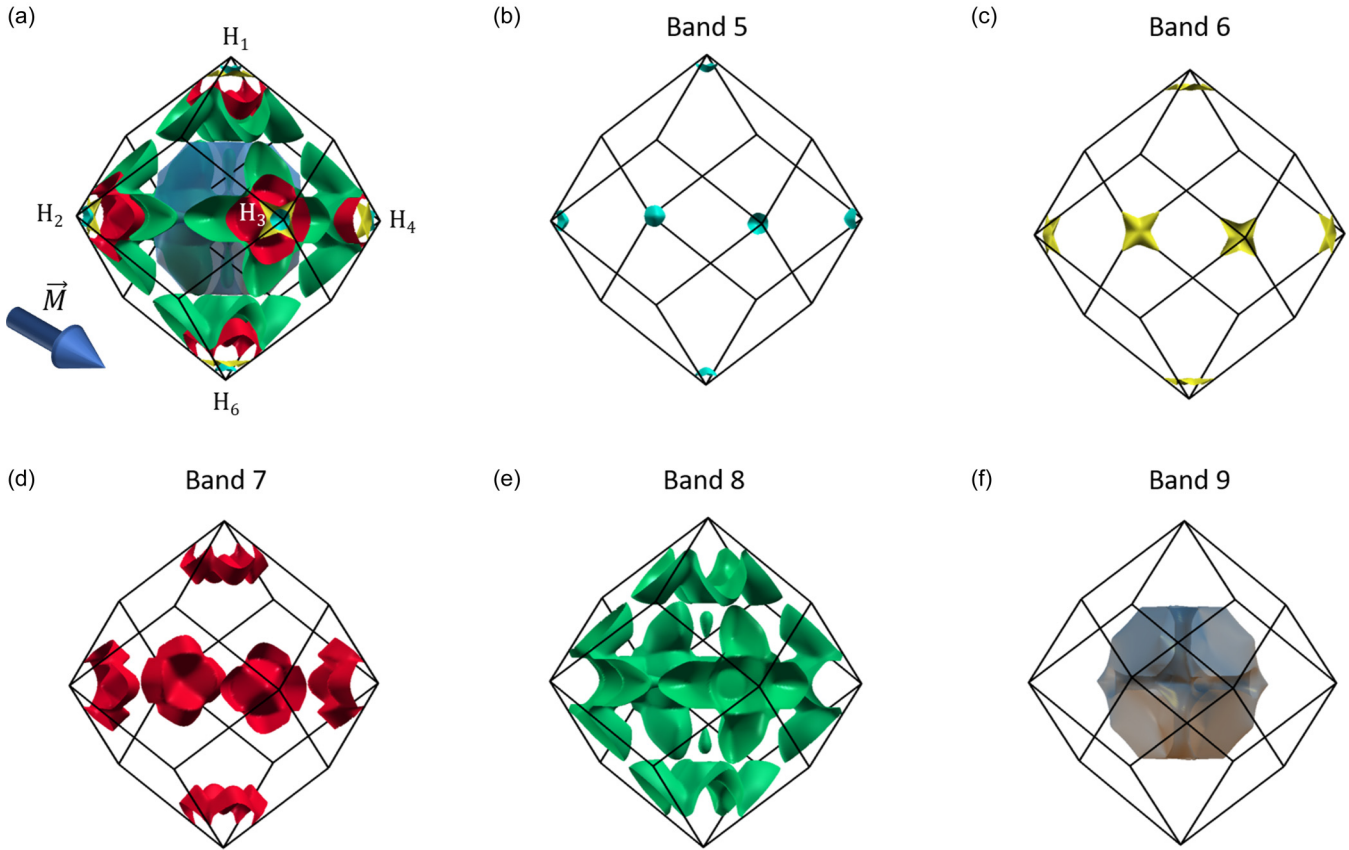
FIG. 2. Theoretical constant energy surfaces of bcc Fe at E_b(\text{GW}) = 0.095 eV with respect to the theoretical Fermi level: (a) superposition of all the bands, (b–f) individual constant energy sheets of bands 5–9. Band 9 is depicted semitransparent. A blue arrow in (a) represents the magnetization direction. The figures were prepared using XCRYSDEN software [41]
