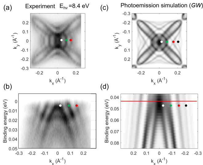
FIG. 7. Comparison of the photoemission intensities obtained using unpolarized light of E_{hv} = 8.4 eV for a 40-ML-thick sample with the photoemission simulation. (a) Experimental constant energy cut near the Fermi level ( E_b = 0.005 eV). (b) Experimental dispersion. (c, d) Results of the photoemission simulation. Red horizontal line in (d) indicates position of the experimental Fermi level. Colored dots indicate corresponding quantum well states.
