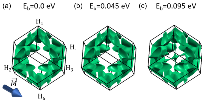
FIG. 3. Constant energy sheets formed by band 8 at different binding energies: (a) E_b = 0.0 eV ( \text{GW} Fermi level), (b) E_b = 0.045 eV (experimental Fermi level), and (c) E_b = 0.095 eV (binding energy of experimental constant energy maps presented in Fig. 4). A blue arrow in (a) represents the magnetization direction. The figures were prepared using XCRYSDEN software [41].
