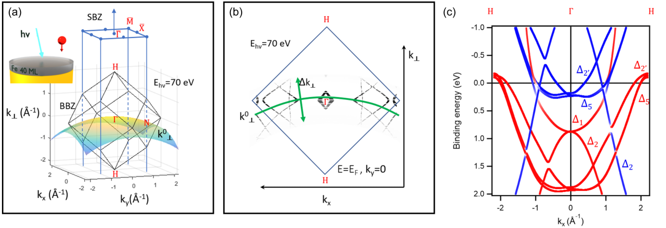
FIG. 1. (a) Bulk Brillouin zone (BBZ) of bcc Fe and surface Brillouin zone (SBZ) of Fe(001) with superimposed k_{\perp}^0(k_x, k_y) surface which defines location of the initial electronic states that contribute to photoemission intensity according to free electron final-state model for photon energy of 70 eV. The inset shows a sketch of the photoemission experiment as seen in real space. (b) Illustration that schematically shows a range of the initial states involved in the photoemission simulation with respect to the size of the BBZ. (c) Relativistic GW bulk electronic structure of bcc Fe along \Delta line of BBZ. Blue (red) color indicates predominantly minority (majority) states. Labels identify orbital symmetry. Negative (positive) k_x values correspond to direction along (perpendicular) to magnetization.
