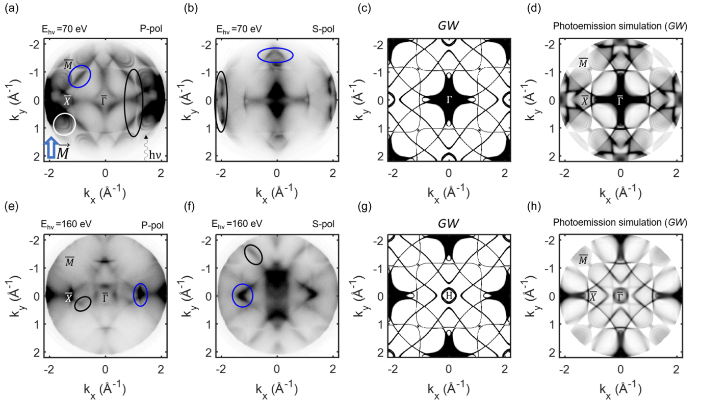
FIG. 4. Comparison of the photoemission intensities obtained using p - and s -polarized light of E_{h\nu} = 70 eV and E_{h\nu} = 160 eV for binding energy of E_b = 0.05 eV for the 40-ML-thick sample with electronic states within a single cut through the k space as defined by FEFSM as well as with the results of the photoemission simulations. (a, b) Experimental result for E_{h\nu} = 70 eV and p - and s -polarized light, respectively. A blue arrow represents the magnetization direction, a wiggly arrow shows the photon incidence direction. (c) Corresponding single cut through the k space, (d) corresponding result of the photoemission simulation. (e, f) Experimental result for E_{h\nu} = 160 eV and p - and s -polarized light, respectively, (g) corresponding single cut through the k space, and (h) corresponding result of the photoemission simulation. Colored ellipsoids mark the features of interest discussed in the text.
