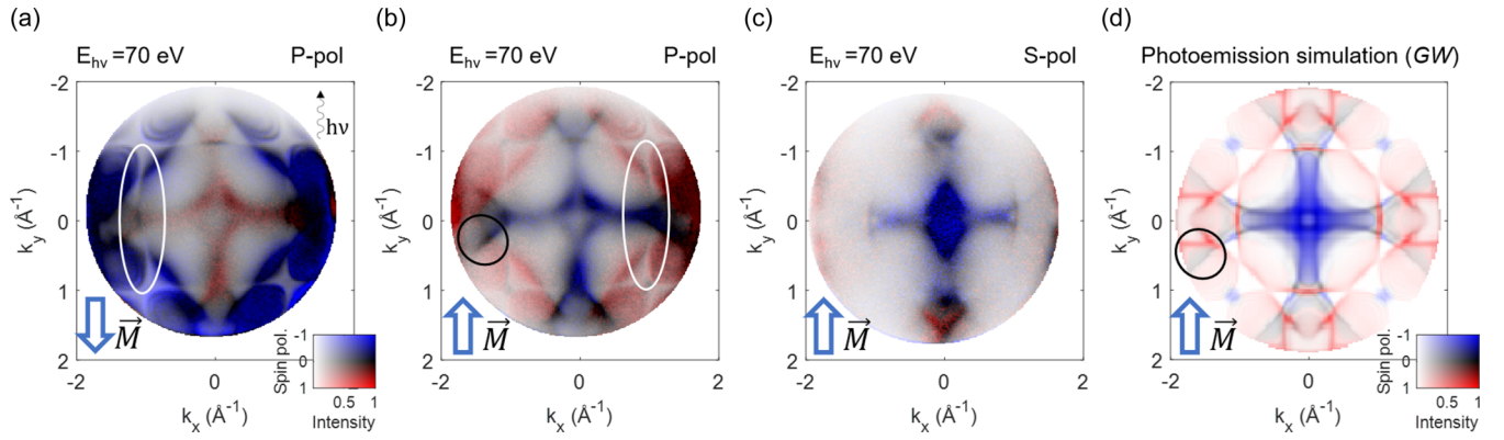
FIG. 6. Comparison of the spin-resolved photoemission intensities with the spin-resolved photoemission simulation. The experimental results are the constant energy cuts ( E_b = 0.1 eV) measured using light of E_{hv} = 70 eV for a 40-ML-thick sample and (a) p polarization when the sample was magnetized DOWN, (b) p polarization when the sample was magnetized UP, and (c) s polarization when the sample was magnetized UP. A wiggly arrow in (a) indicates the photon incidence direction. (d) Result of the spin-polarized photoemission simulation. The two-dimensional color map shown in the insets is the same for all the figures. Blue and red color in (b–d) indicate predominantly minority and majority spin states, respectively. Black and white ellipses indicate features of interest discussed in the text.
