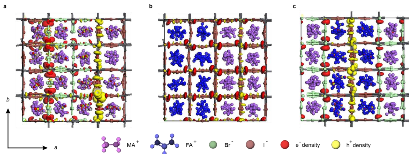
Fig. 4 | DFT- and TDDFT-calculations reveal driving force for mixed-halide mediated charge separation. a , Charge densities of the lowest excited-state geometry relaxed from the optimised ground-state geometry of MAPbI 3 /MAPbBr 3 heterojunction along the a axis, showing charge localisation across the Br – I heterojunction. b , Charge densities of the lowest excited-state geometry relaxed from the optimised ground-state geometry of FAPbI 3 /MAPbI 3 heterojunction along a axis, displaying no additional driving force for charge segregation across the heterojunction. c , Charge densities of the lowest excited-state geometry relaxed from the optimised ground-state geometry of FAPbI 3 /MAPbBr 3 heterojunction along a axis, displaying no additional driving force for charge segregation across the heterojunction.
