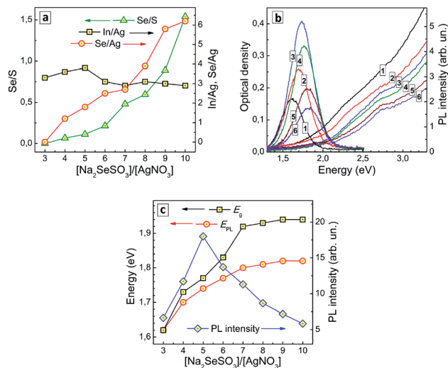
Fig. 4 (a) Atomic ratios of Se to S (triangles), In to Ag (squares), and Se to Ag (circles) as functions of the nominal ratio of molar concentrations of Na_2SeSO_3 and AgNO_3 during the QD synthesis. (b) Absorption and PL spectra of AISE QDs produced at a different [SS]/[Ag] ratios of 3 (curves 1), 4 (2), 5 (3), 7 (4), 8 (5), and 10 (6). (c) Bandgap (squares), PL band maximum energy (circles), and PL intensity (diamonds) as functions of the [SS]/[Ag] ratio. Lines connecting the points in (a) and (c) are guides for the eye only.
