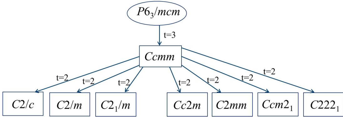
Figure 6.3: A schematic drawing illustrating the group-subgroup relationships relevant for the refinements.
