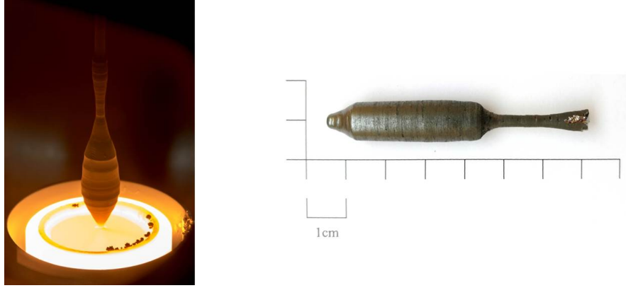
Figure 3.4: Photo showing the growth of the single crystal and a picture of the final \text{Mn}_5\text{Ge}_3 crystal.
