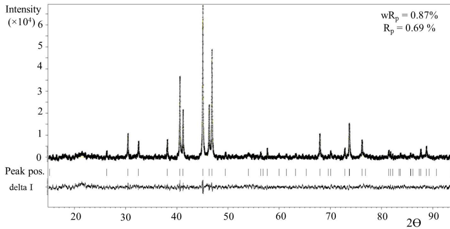
Figure A.5: Observed intensities and the difference profile of \text{MnFe}_4\text{Si}_3 measured at room temperature from the LeBail refinement
