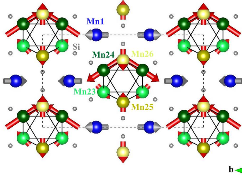
Figure 6.7: Schematic representation of the magnetic structure projected along the c -direction based on the refinement in magnetic space group P[C]2an . The arrows indicate the magnitude and the direction of the ordered moments.
