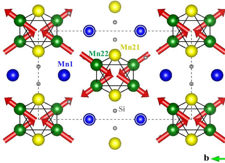
Figure 6.6: Schematic representation of the magnetic structure projected along the c -direction based on the refinement in the magnetic space group P[C]_{can} . The arrows indicate the magnitude and the direction of the ordered moments.
