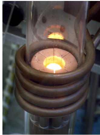
Figure 3.2: Photo of the melting process of the material in the cold crucible induction melting [taken from [95]].
