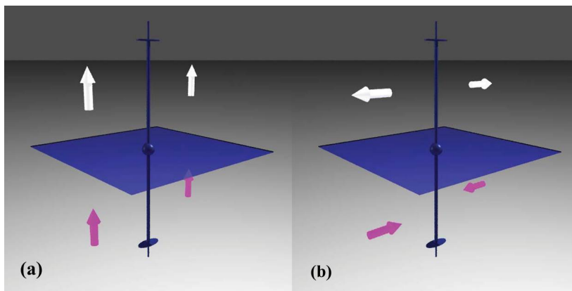
Figure 2.5: Representation of the operations of the point group 2/m on an axial vector, oriented parallel to the twofold axis (a) and parallel to the mirror plane (b) [taken from [87]].
