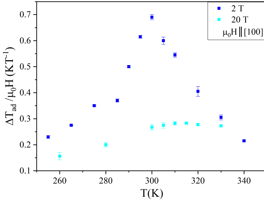
Figure 4.10: \Delta T_{ad} / \mu_0 H for a field of 2 and 20 T parallel to [100] direction.
