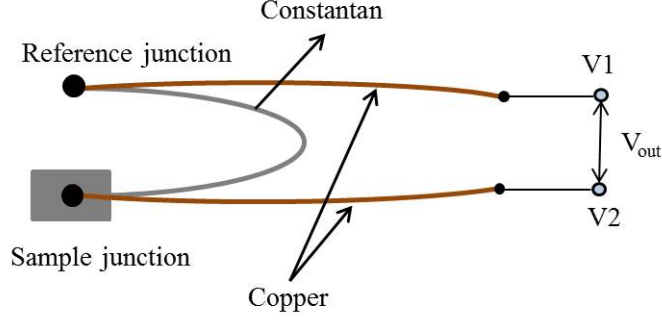
Figure 3.13: Schematic drawing the differential copper-constantan thermocouple [modified from [35]].
