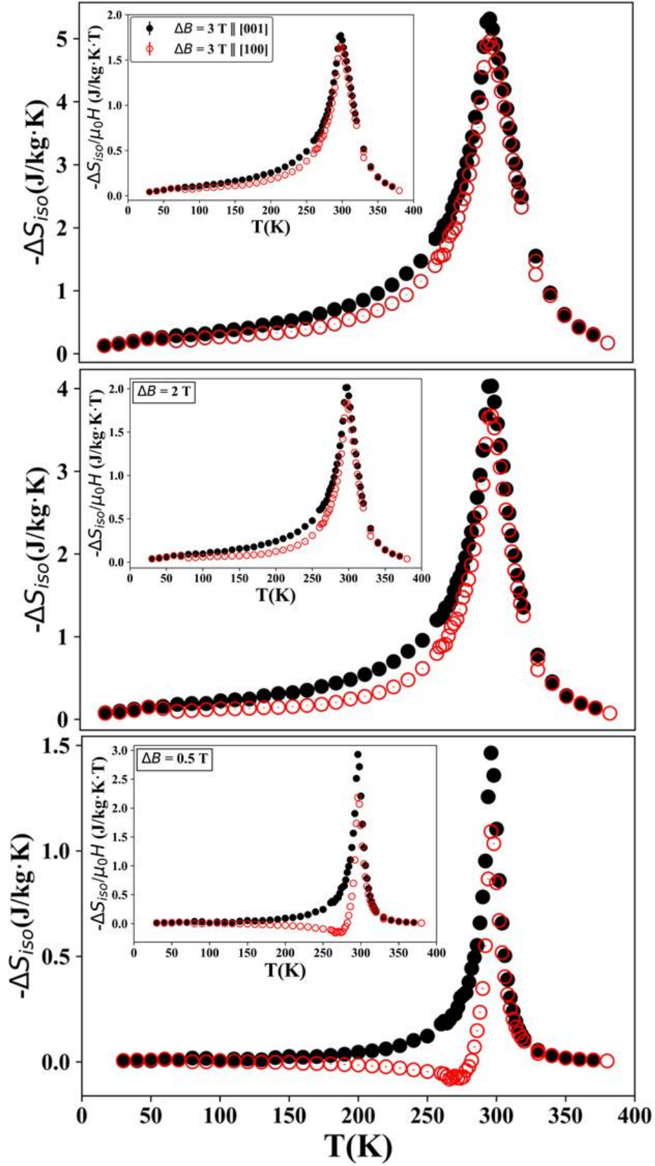
Figure 5.8: Magnetic entropy change of Mn_5Ge_3 determined from magnetization data at a field of 0.5, 2 and 3 T parallel to [001] (black closed symbol) and [100] (red opened symbol) directions. The insets show -\Delta S_{iso}/\mu_0 H for all curves.
