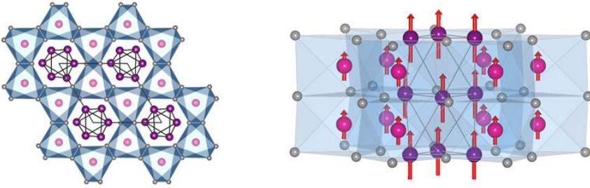
Figure 1.6: (Left) Projection of Mn 5 Ge 3 structure in space group P6_3/mcm along the [001]-direction. Sites occupied by Mn1 are shown in pink (4 d ), sites occupied by Mn2 are shown in magenta (6 g ); Ge atoms are shown in grey (6 g ) and [MnGe 6 ]-octahedra are indicated in blue. (Right) Schematic diagram illustrating the ferromagnetic structure of Mn 5 Ge 3 , projection slightly tilted from the [110]-direction. The length of the arrows corresponds to M = 1.96(3) \mu_B and 3.23(2) \mu_B for the 4 d and 6 g sites, respectively [taken from [51]].
