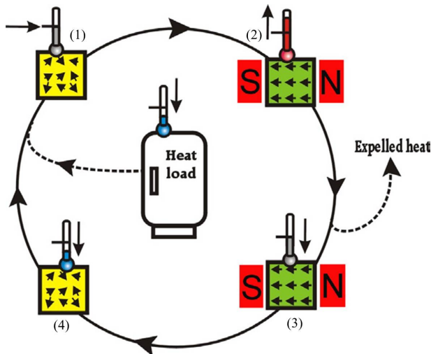
Figure 1.2: Schematic of a magnetic-refrigeration cycle [taken from [31]].
