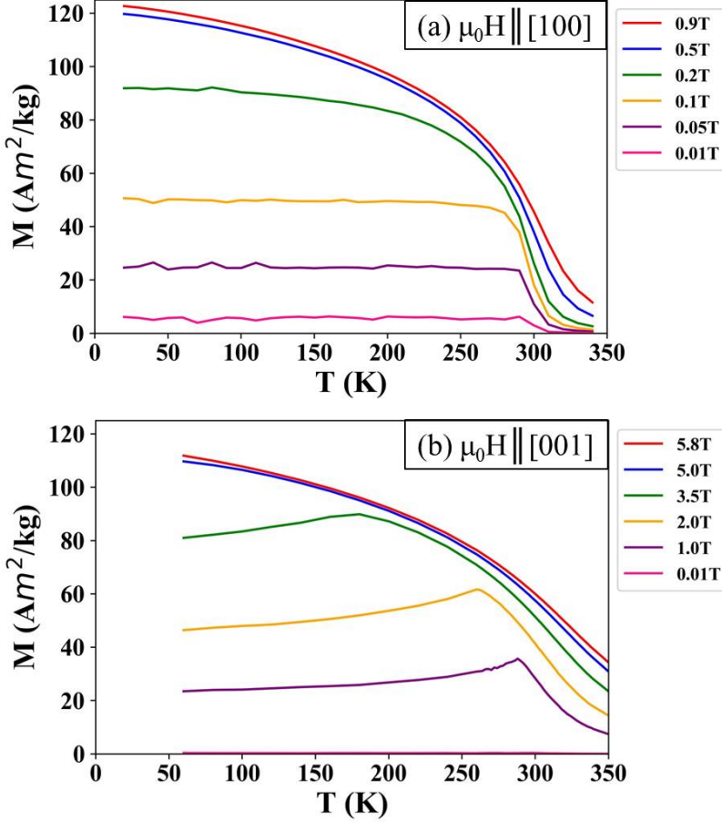
Figure 4.3: Temperature-dependent magnetization of \text{MnFe}_4\text{Si}_3 from hysteresis measurements, for \vec{H} \parallel [100] (a) and \vec{H} \parallel [001] (b).
