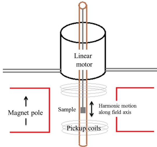
Figure 3.8: Basic schematic of VSM set-up [taken from [107]].
