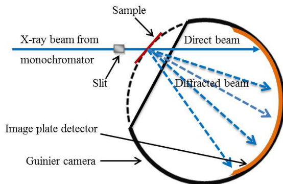
Figure 3.5: Schematic representation of the powder diffractometer setup with Guinier geometry [modified from [99]].
