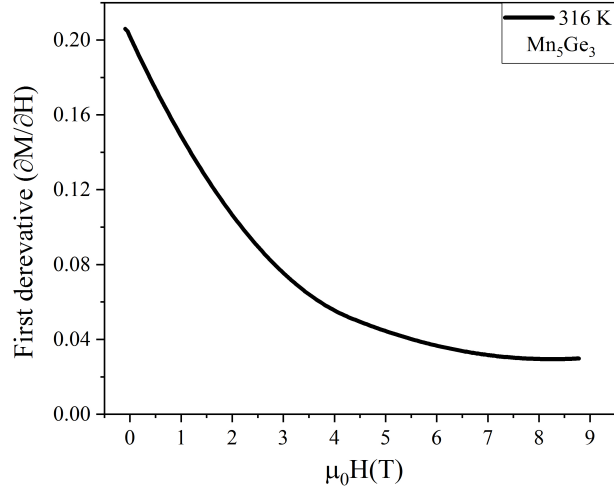
Figure A.3: The first derivative (\partial M / \partial H) for the interpolated M(H) curve at 316 K vs. the interpolated field H .
