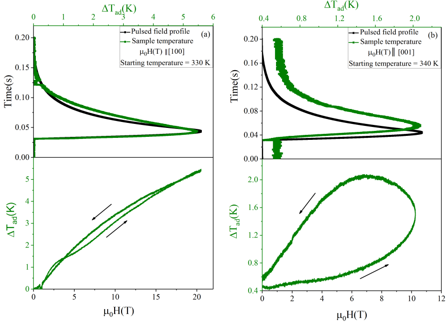
Figure 4.7: Field and time dependence of \Delta T_{ad} for a pulsed magnetic field of (a) 20 T applied along the [100] direction at 330 K (b) 10 T applied along the [001] direction at 340 K.
