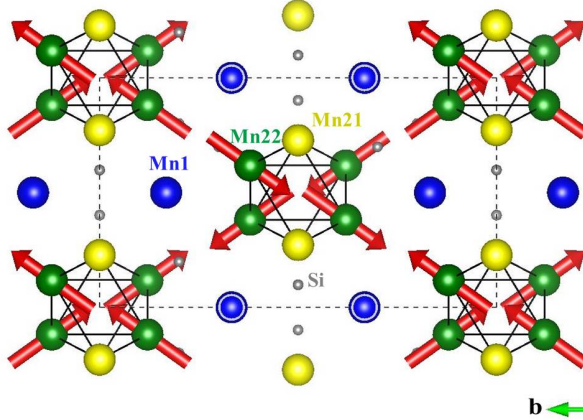
Figure 6.6: Schematic representation of the magnetic structure projected along the c -direction based on the refinement in the magnetic space group P[C]can . The arrows indicate the magnitude and the direction of the ordered moments.
