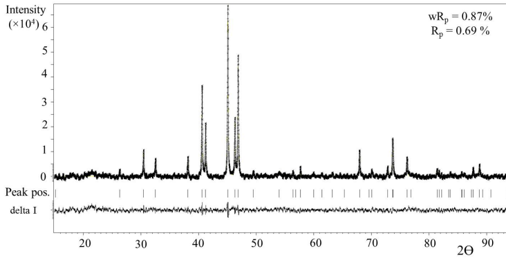
Figure A.5: Observed intensities and the difference profile of MnFe_4Si_3 measured at room temperature from the LeBail refinement
