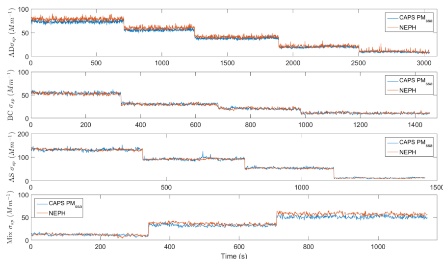
Figure 7. Time series of the measurements by the scattering channel.
