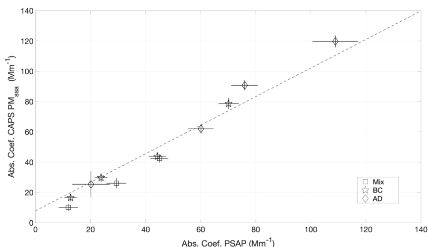
Figure 11. Comparison result of the absorption indirect measurement by the CAPS \text{PM}_{\text{ssa}} with the measurements from the PSAP for AD, BC and Mixture.
