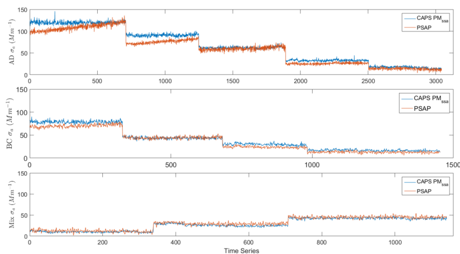
Figure 10. Time series of the measurements by the absorption channel.
