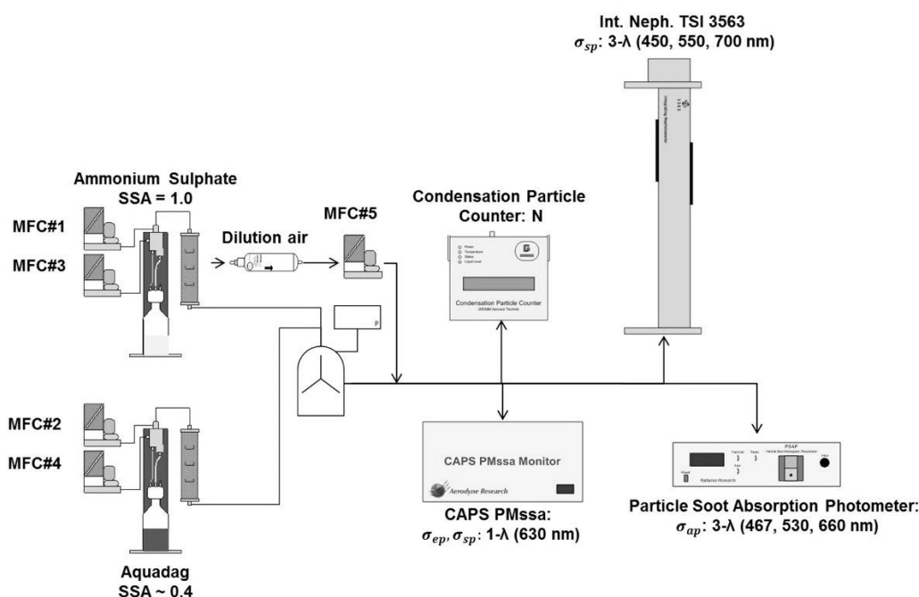
Figure 1. Instrumental set-up applied in the optical closure study
