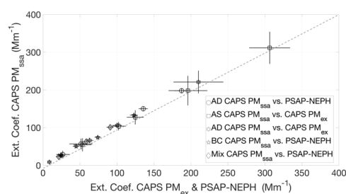
Figure 4. Comparison result of the extinction channel of the CAPS PM_{ssa} with the CAPS PM_{ex} and the PSAP-NEPH for the different aerosol types.
