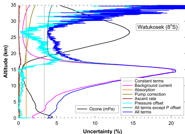
Figure 10. Uncertainty analysis for a tropical station (Watakosek, Java), showing the influence of different uncertainty terms, for the assumed values in Table 2. Because of the very low ozone in the tropical upper troposphere, the uncertainty due to the background current dominates at these altitudes.
