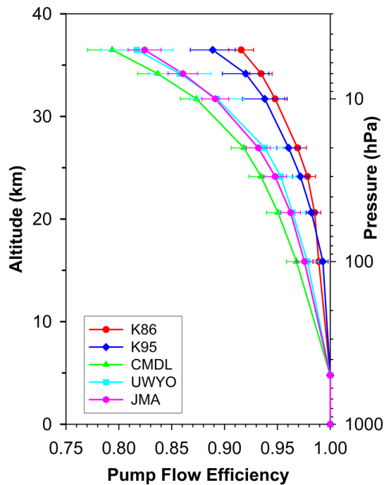
Figure 3. Pump flow efficiencies ( \eta_p ) as a function of air pressure for ECC-ozone sondes reported by Komhyr (1986), Komhyr et al. (1995), Johnson et al. (2002); (CMDL and UWYO), and Nakano, personal communication, 2019) (JMA). See also Table S2 in the supporting information.
