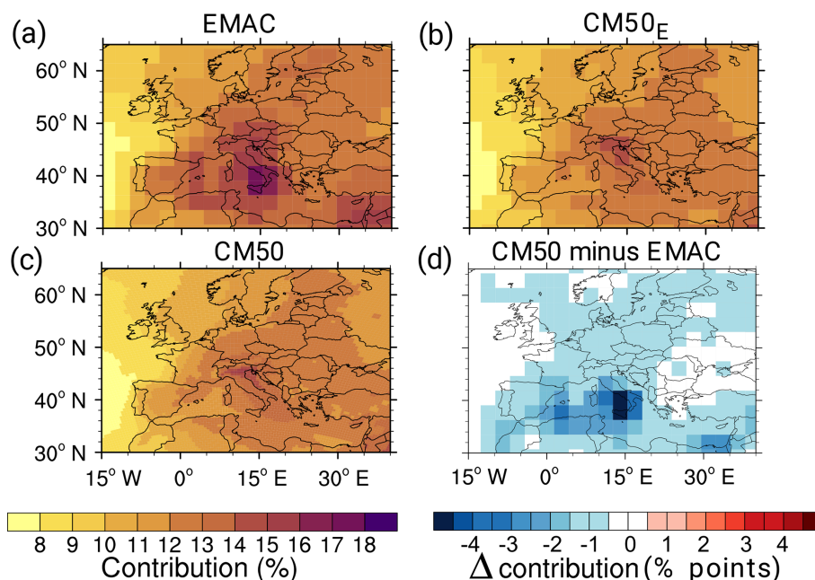
Figure 8. Comparison of the JJA average relative contribution of \text{O}_3^{\text{tra}} to ground-level \text{O}_3 (in percent) of EMAC and CM50: (a) results of EMAC, (b) results of CM50 transformed onto the EMAC grid, (c) results of CM50 on the original grid, and (d) difference (“CM50 minus EMAC” in percentage points) on the coarse grid. The comparisons in (a–c) use the same scale. Shown are the results of the REF simulation, averaged over 2008–2010.
