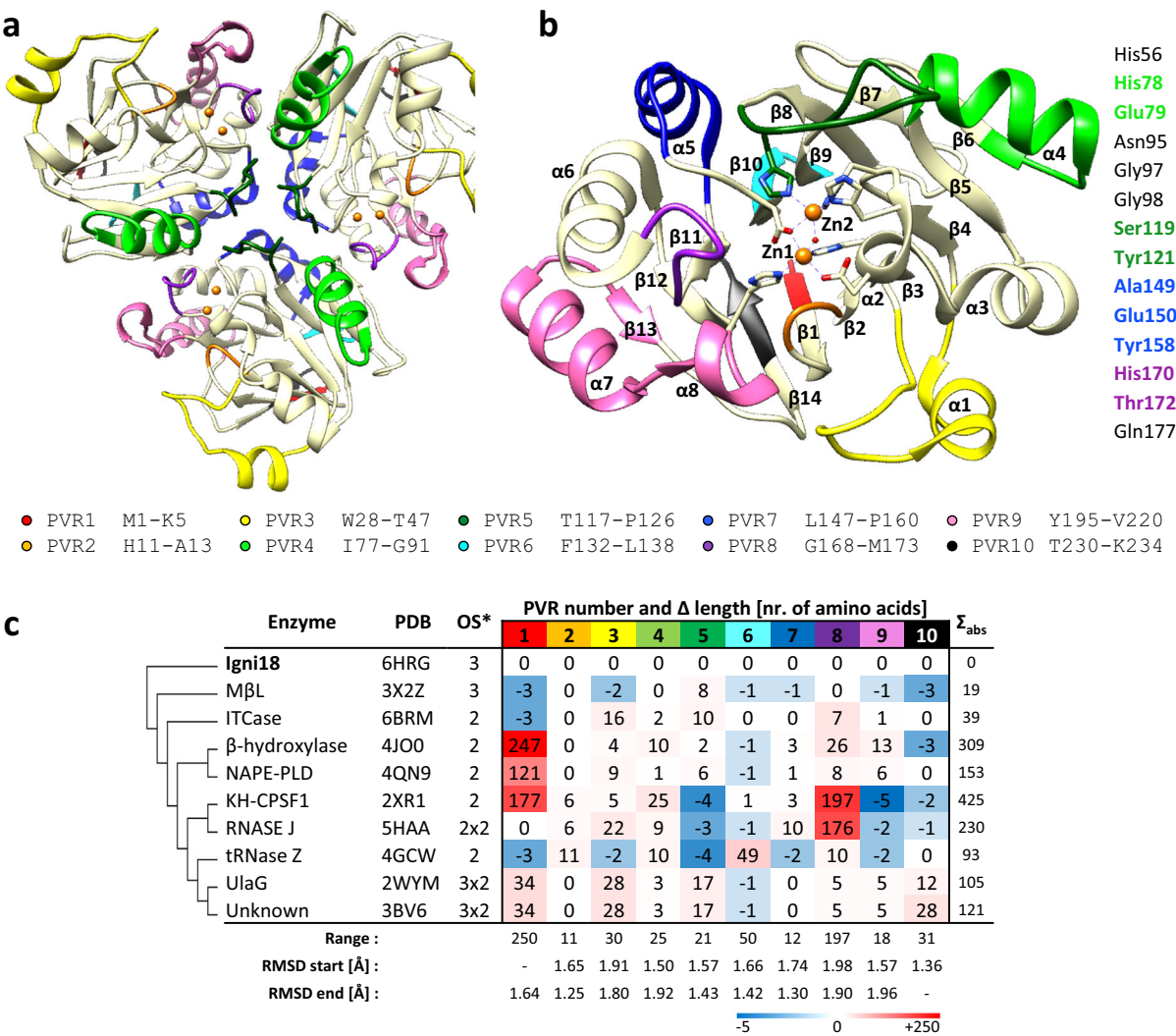
Fig. 1 The crystal structure of Igni18 reveals the origin of diverse MβLs. The protein crystalized as a homotrimer (a). A monomer (b) comprises 8 α-helices and 14 β-strands and contains two Zn 2+ ions (orange). Ten Protein Variable Regions (PVRs) describe structural evolution and specialization within the MβL family and are depicted in a and b. The amino acids comprising each PVR are indicated underneath. In total, 9 out of 14 amino acids needed for stabilization of the trimer are found within PVRs 4, 5, 7, and 8 (light-green, dark-green, blue, and purple; right), leading to an evolutionary fast loss of this quaternary structure. Differences in the number of amino acids of the described PVRs among 10 MβL-fold-containing structures (c): Molecular relation (left) and absolute variation in the number of amino acids (Σ abs , right) compared to Igni18 as well as statistic data on PVR descriptors (total length range > 10 amino acids, start/end position RMSDs for all aligned structures <2 Å; bottom) are also given. Asterisk represents Oligomerization state of the crystallized enzyme (3: trimer; 2: dimer; 2 × 2: double dimer; 3 × 2: triple dimer).
