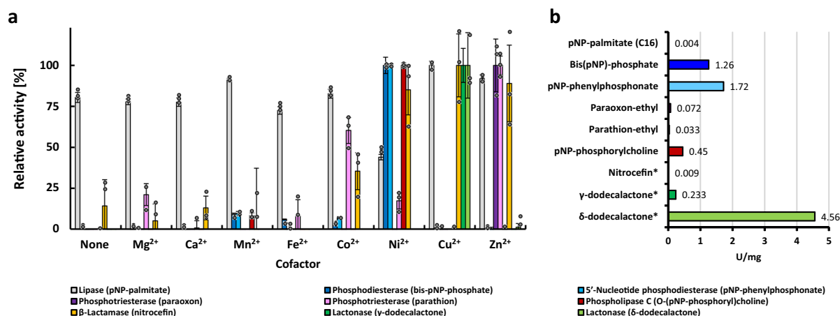
Fig. 3 Different divalent metal ions drive Igni18's enzymatic promiscuity. a Metal-dependency of Igni18 was measured with nine substrates representing activities catalyzed by MβLs. All activities but lipase showed a strict metal dependency. Error bars represent the relative standard deviation ( n = 3 independent experiments). b Absolute activities measured in \text{U mg}^{-1} under optimal conditions but the ones marked with an asterisk, which were measured at 40^\circ\text{C} (see Methods section).
