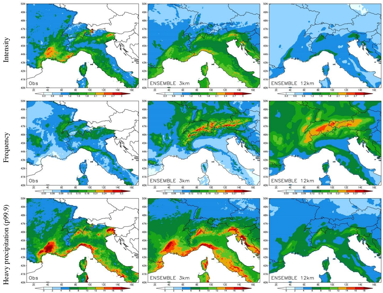
Figure 3 As Fig. 2 but for autumn hourly precipitation (mm/h).
