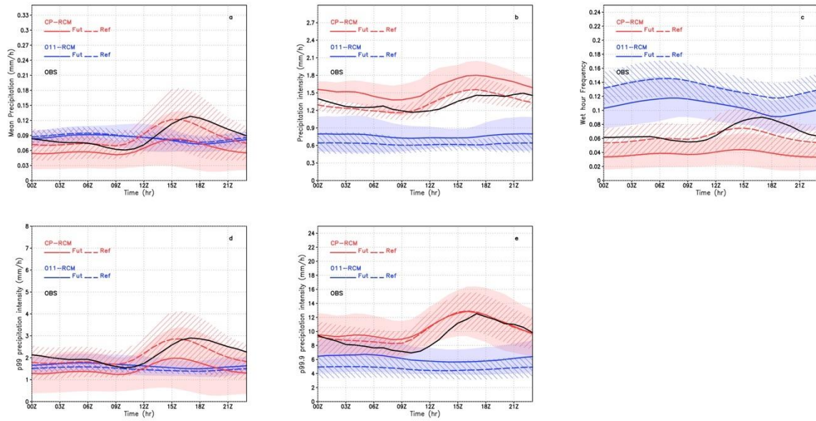
Figure 7 As in Fig. 5 but averaged over France and with the observed COMEPHORE data (black, section 4).
