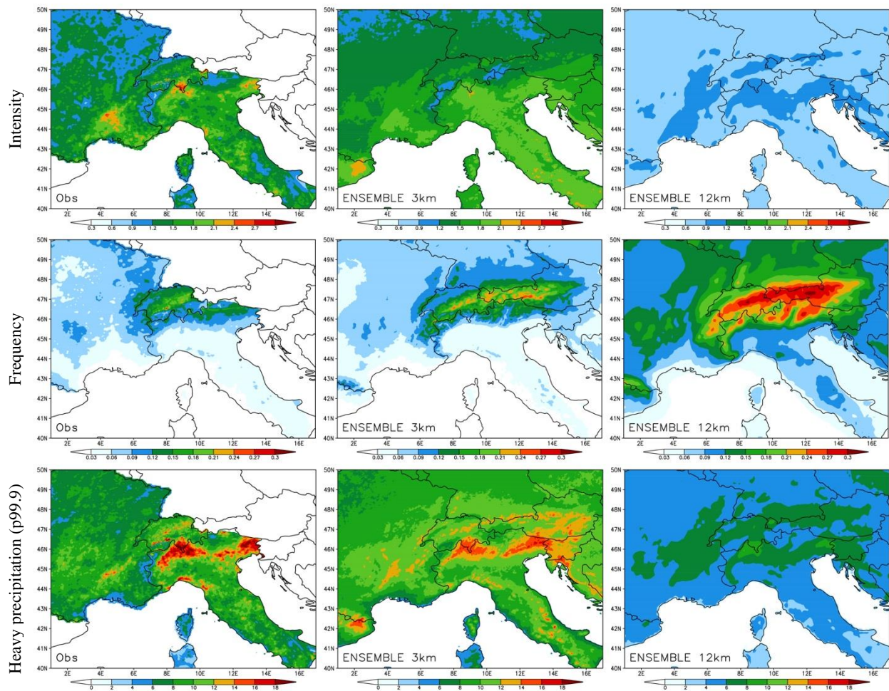
Figure 2 Summer hourly indices over the Alpine region. From top to bottom: intensity of hourly precipitation (mm/h), wet-hour frequency, heavy hourly precipitation (mm/h) events (p99.9). Results are obtained (from left to right) by a combination of high resolution observations over different areas (see section 4 for details and considered periods), the ensemble of CPRCMs and the ensemble of the corresponding driving RCMs. The model results are averaged over the period 1996-2005.
