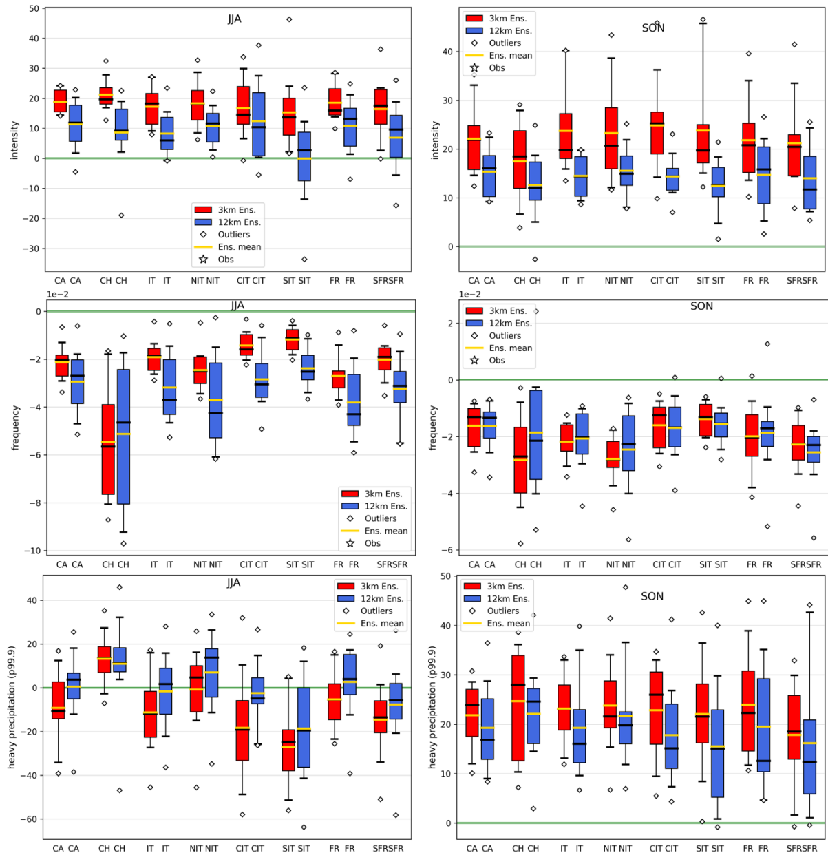
Figure 11 JJA (left) and SON (right) box-plot representing the distribution of the percent change signal within the population of the CPRCM (red) and driving RCM (blue) ensembles over different areas (CA: common domain area as in Fig. 1, CH: Switzerland, (N/C/S)IT:(North/Central/South) Italy, (S)FR: (South) France) over 2090-99. The distribution is represented within the 5th and 95 percentile, for (from top to bottom) mean wet-hour intensity, wet-hour frequency, heavy hourly precipitation (p99.9). Outliers are represented singularly (open diamonds); the zero is plotted in green.
