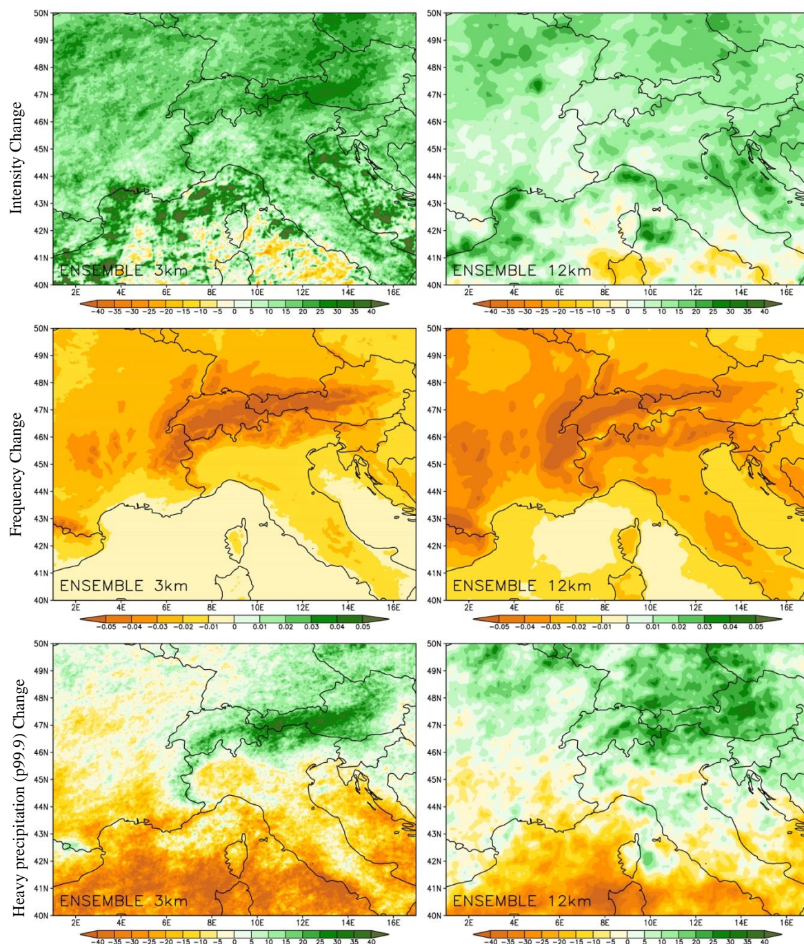
Figure 9 Ensemble mean percent change of the indices analysed over 2090-2099 for the summer hourly precipitation (historical simulation is the reference, 1996-2005). From top to bottom: intensity, frequency (change) and heavy precipitation (p99.9). The results are obtained from the CPRCM ensemble (left) and the driving RCM ensemble (right).
