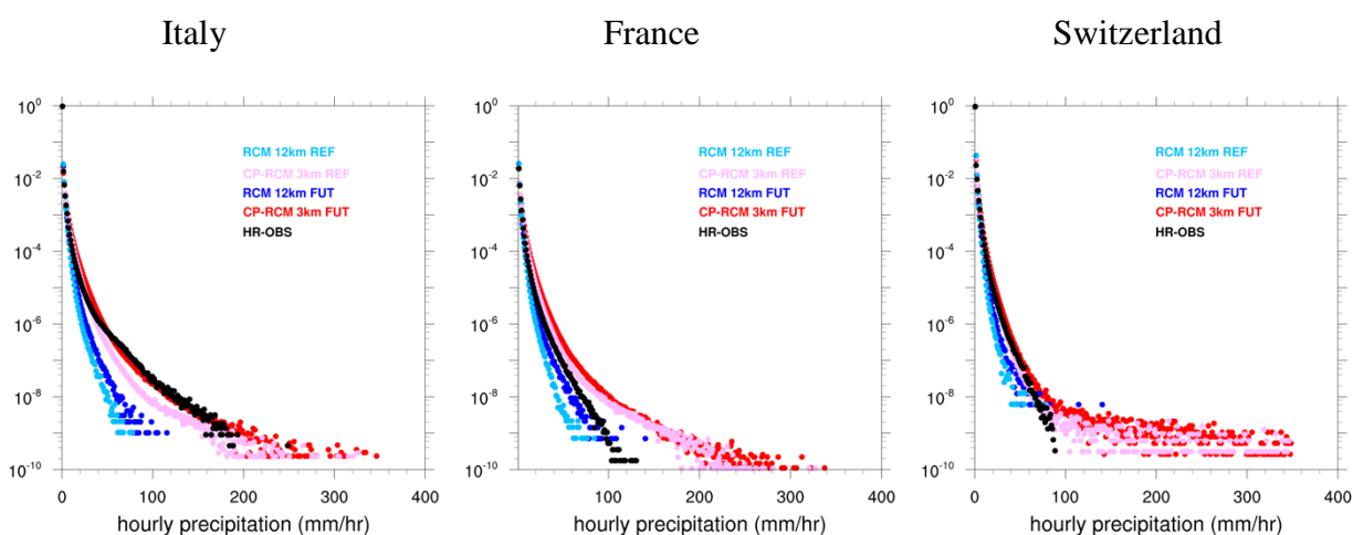
Figure 8 Probability density function (PDF) of hourly precipitation (mm/h) over Italy (left), France (middle) and Switzerland (right) for the highest-resolution observed data over the historical decade (black, section 4; GRIPHO for Italy, COMEPHORE for France, RdisaggH for Switzerland); for the CPRCM (pink for 1996-2005 and red for 2090-2099) and the driving RCM (light blue for 1996-2005 and blue for 2090-2099) ensembles.
