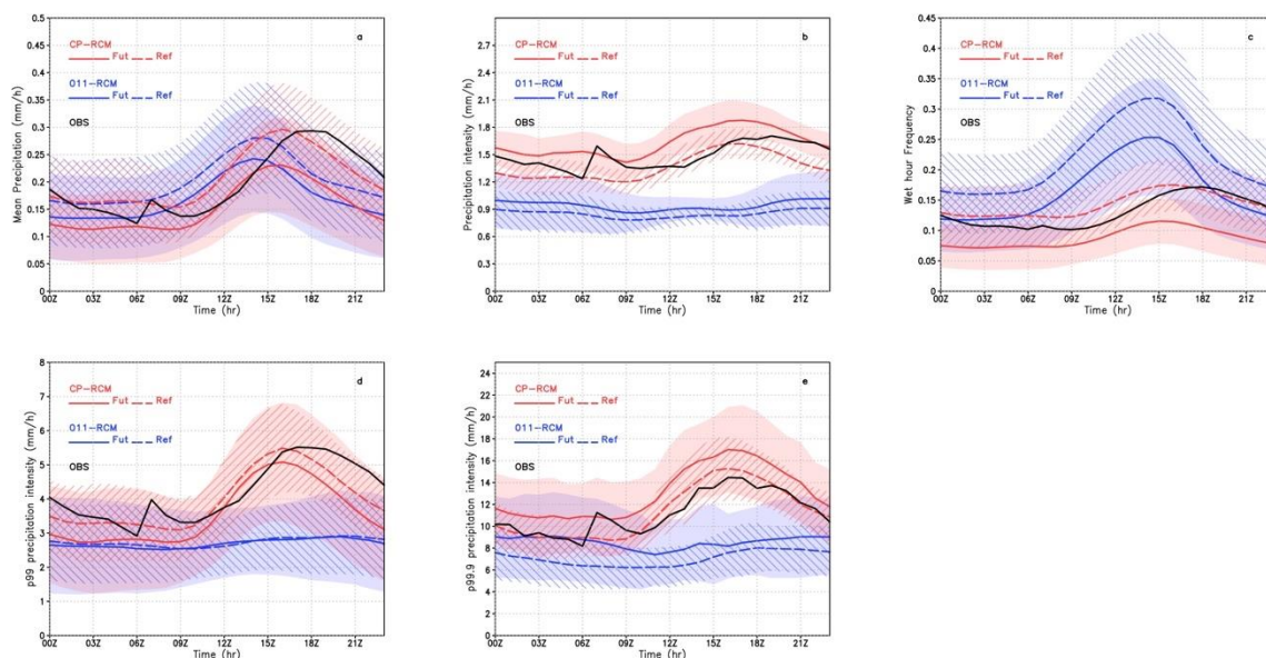
Figure 5 Summer diurnal cycle of mean hourly precipitation (a, mm/h), hourly intensity precipitation (b, mm/h), wet-hour frequency (c), heavy hourly precipitation (p99 (d); p99.9 (e), mm/h) averaged over Switzerland. The black line reports the observations (black, RdisaggH dataset, section 4); lines and corresponding shaded areas represent the ensemble mean and standard deviation of the CPRCMs simulations (red) and of the corresponding driving RCMs simulations (blue) for the decade 2090-2099 (solid line and plain colour area) and for the reference period 1996-2005 (dashed line and diagonal lines area).
