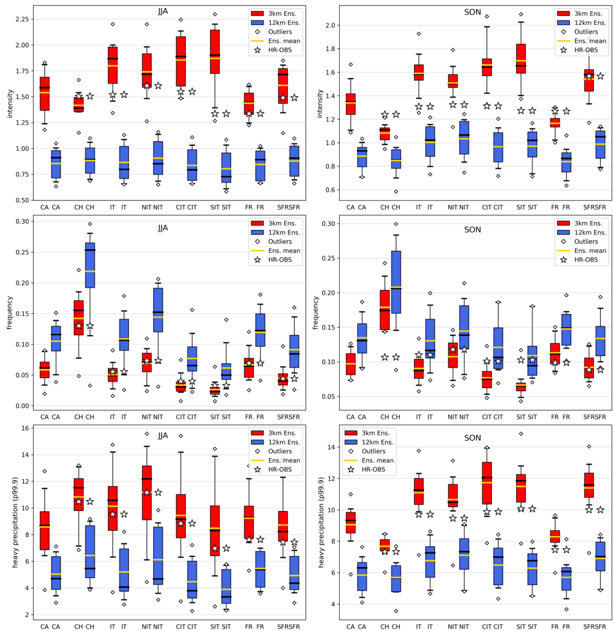
Figure 4 JJA (left) and SON (right) box-plot representing the distribution of the CPRCM (red) and driving RCM (blue) ensemble members over different areas (CA: common domain as represented in Fig. 1, CH: Switzerland, (N/C/S)IT:(North/Central/South) Italy, (S)FR: (South) France) over the historical period 1996-2005. The distribution is represented within 5th and 95 percentile, for (from top to bottom) mean wet-hour intensity (mm/h), wet-hour frequency, heavy hourly precipitation (p99.9, mm/h). Outliers are represented singularly (open diamonds), ensemble mean (yellow line) is also reported and compared with the highest resolution observations (white star) over the same area (Table 4).
