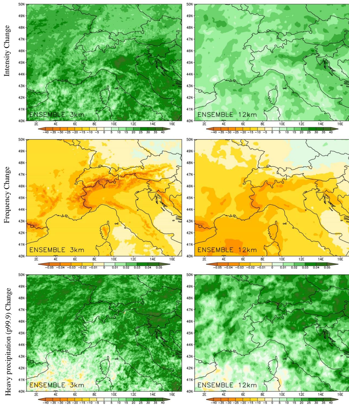
Figure 10 Same as Fig 9 but for autumn hourly precipitation mean change
