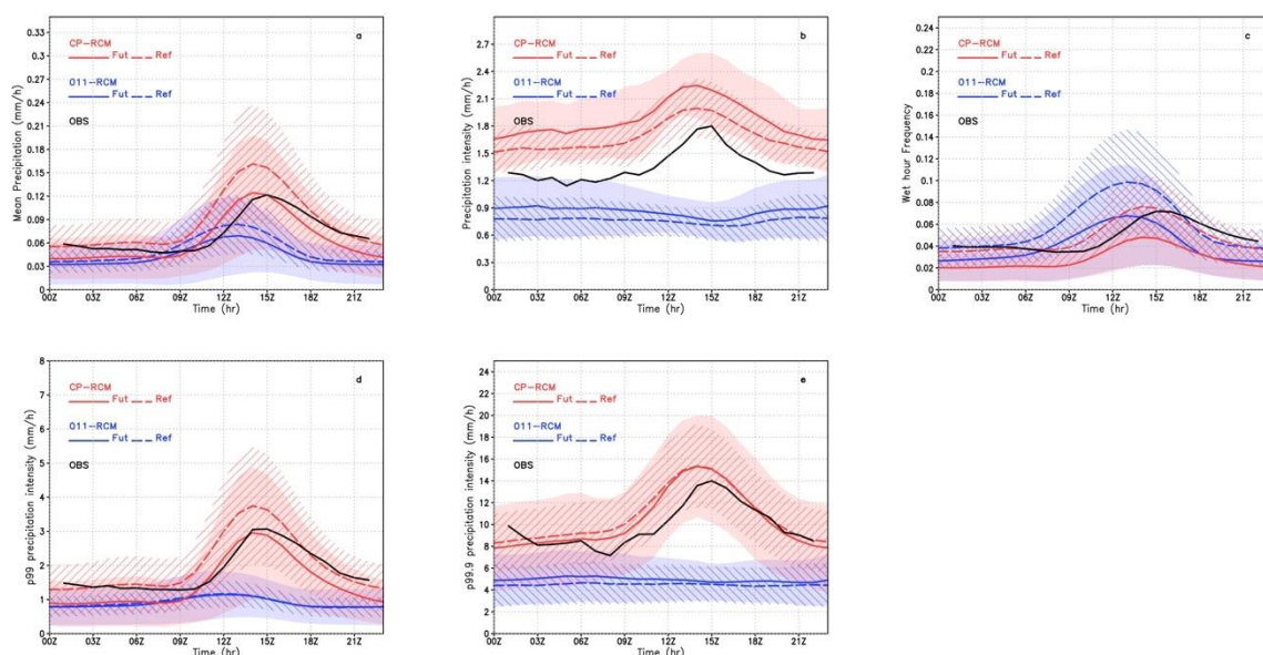
Figure 6 As in Fig. 5 but averaged over Italy and with the observed GRIPHO data (black, section 4).
