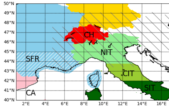
Figure 1 Common domain (CA). Areas where observed dataset are available (section 4) are in different colours: EURO4M-APGD (dashed grey), REGNIE (yellow), Spain02 (pink), RdisaggH (red), COMEPHORE (blue), GRIPHO (greenish). Sub-domain areas considered in the analysis are labelled: South France (SFR), North, Central, South Italy (N/C/SIT), Switzerland (CH).
