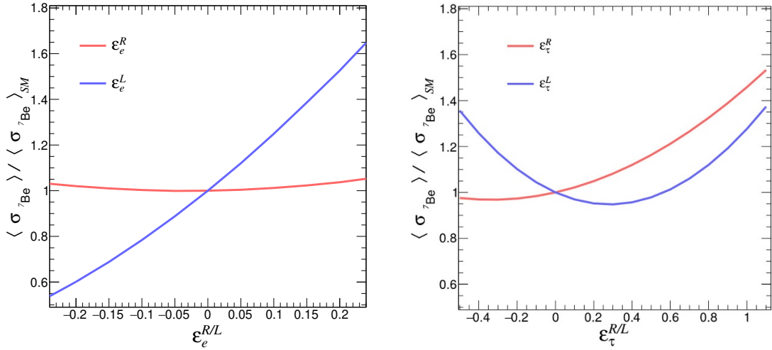
Figure 3. The relative change of the total cross section ratio \langle\sigma_{7\text{Be}}\rangle/\langle\sigma_{7\text{Be}}\rangle_{\text{SM}} as function of \varepsilon_e^{R/L} (left panel) and \varepsilon_\tau^{R/L} (right panel).
