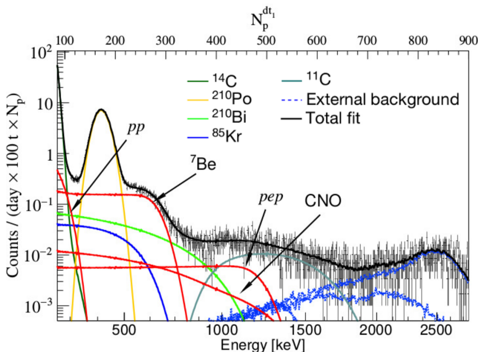
Figure 4. Example of fit of the Borexino energy spectrum. The fit was performed using the N_p^{dt1} energy estimator. The bottom horizontal axis has been converted from N_p^{dt1} into units of energy; N_p is a number of photoelectrons in the acquisition time window.
