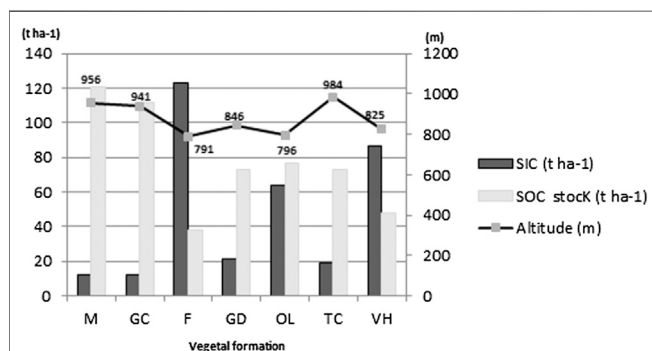
FIGURE 2 | SOC stocks variation according to SIC (CaCO 3 ) and altitude. M: matorral; GC: sparse garrigue; F: forest; GD: dense garrigue; OL: olive grove; TC: oak coppice; VH: herbaceous vegetation.
