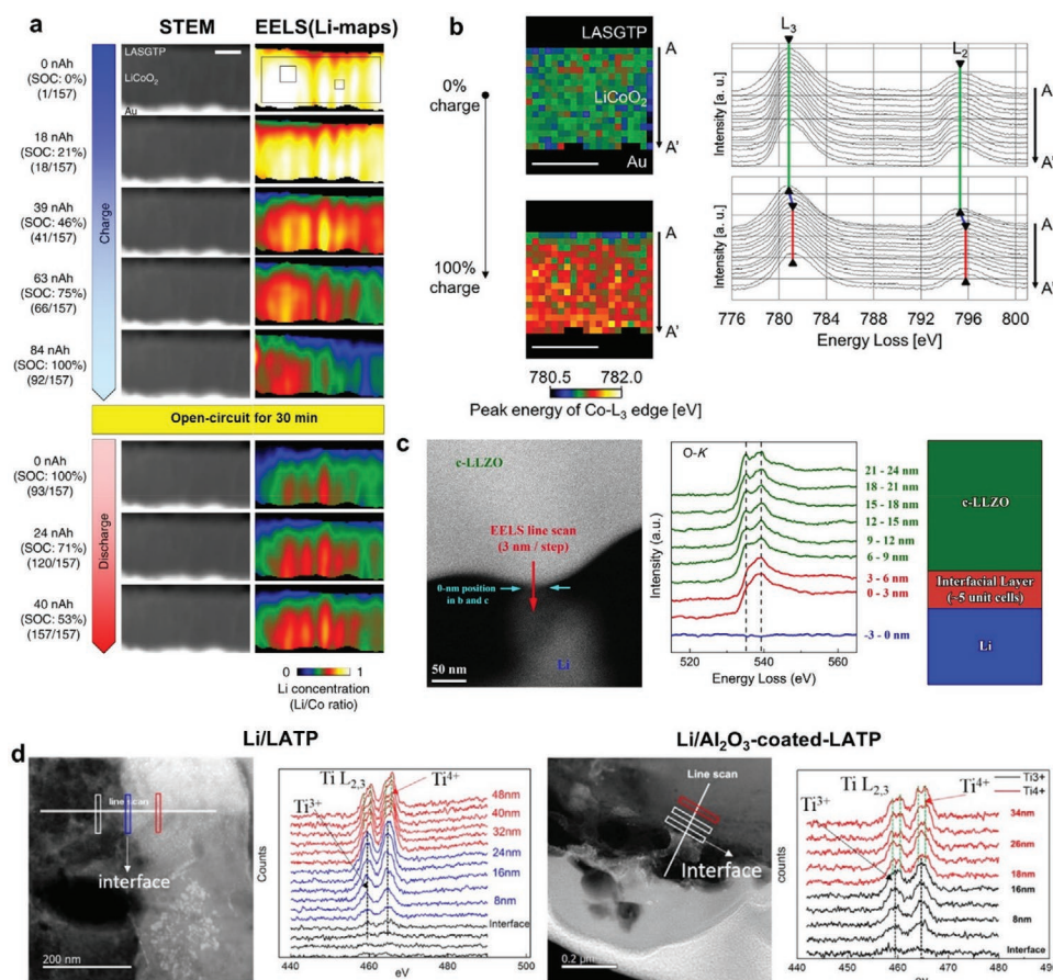
Figure 21. In situ STEM and EELS measurement of the \text{LiCoO}_2/\text{Li}_{1-x+y}\text{Al}_x(\text{Ti,Ge})_{2-x-y}\text{Si}_{3-y}\text{O}_{12} interface at different SoC a). Peak position maps of the Co-L 3 edge and the corresponding EELS spectra of Co-L 2,3 from position A to A' across the \text{LiCoO}_2/\text{Li}_{1-x+y}\text{Al}_x(\text{Ti,Ge})_{2-x-y}\text{Si}_{3-y}\text{O}_{12} interface at pristine and fully charged state b). HAADF-STEM image of the \text{Li}/\text{Li}_{1-3x}\text{Al}_x\text{La}_3\text{Zr}_2\text{O}_{12} interface and corresponding O-K edge EELS line scan results c). HRTEM image of the \text{Li}/\text{Li}_{1.3}\text{Al}_{0.3}\text{Ti}_{1.7}(\text{PO}_4)_3 interface and corresponding Ti L 2,3 -edge EELS line scan for bare and \text{Al}_2\text{O}_3 -coated samples d). a) Reproduced with permission. [261] Copyright 2020, Springer-Nature. b) Reproduced with permission. [262] Copyright 2018, American Chemical Society. c) Reproduced with permission. [265] Copyright 2016, American Chemical Society. d) Reproduced with permission. [153] Copyright 2018, American Chemical Society.
