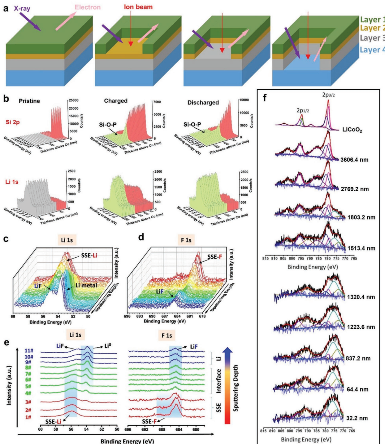
Figure 12. Schematic illustration of sputter-etched XPS measurement for layered samples a). Si, Li spectra at the Si/Li 3 PO 4 /LiCoO 2 ASSB. Signals from the Si and Li 3 PO 4 layer are respectively shown in red and gray. The newly formed interlayer is shown in green b). Li and F spectra of the Li/Li 6 PS 5 Cl 0.3 F 0.7 interface c–e). Co spectra of the Li 7 La 3 Zr 2 O 12 /LiCoO 2 interface f). b) Reproduced with permission. [4] Copyright 2018, Wiley-VCH. c–e) Reproduced with permission. [208] Copyright 2020, American Chemical Society. f) Reproduced with permission. [209] Copyright 2017, IOP publishing.
