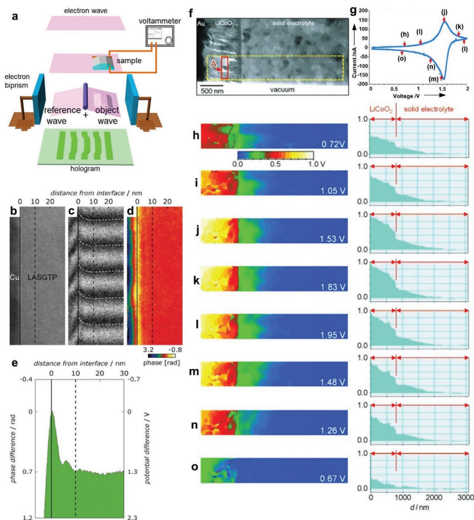
Figure 22. Schematic illustration of the EH working principle a). Cross-sectional TEM image b), corresponding hologram image c) and reconstructed phase map d) at the \text{Cu}/\text{Li}_{1+x+y}\text{Al}_x\text{Ti}_{2-x}\text{Si}_{3-y}\text{O}_{12} interface. The phase-potential profile in (e) was generated by integrating along the vertical direction of (d). Bright-field TEM image at the \text{LiCoO}_2/\text{Li}_{1+x+y}\text{Al}_x\text{Ti}_{2-x}\text{Si}_{3-y}\text{O}_{12} interface f). CV curve for the in situ EH measurement g). 2D potential images (left) and corresponding line profiles (right) during the charging-discharging process h–o). a) Reproduced with permission. [259] Copyright 2016, Oxford University Press. b–e) Reproduced with permission. [274] Copyright 2019, Wiley-VCH. f–o) Reproduced with permission. [277] Copyright 2010, Wiley-VCH.
