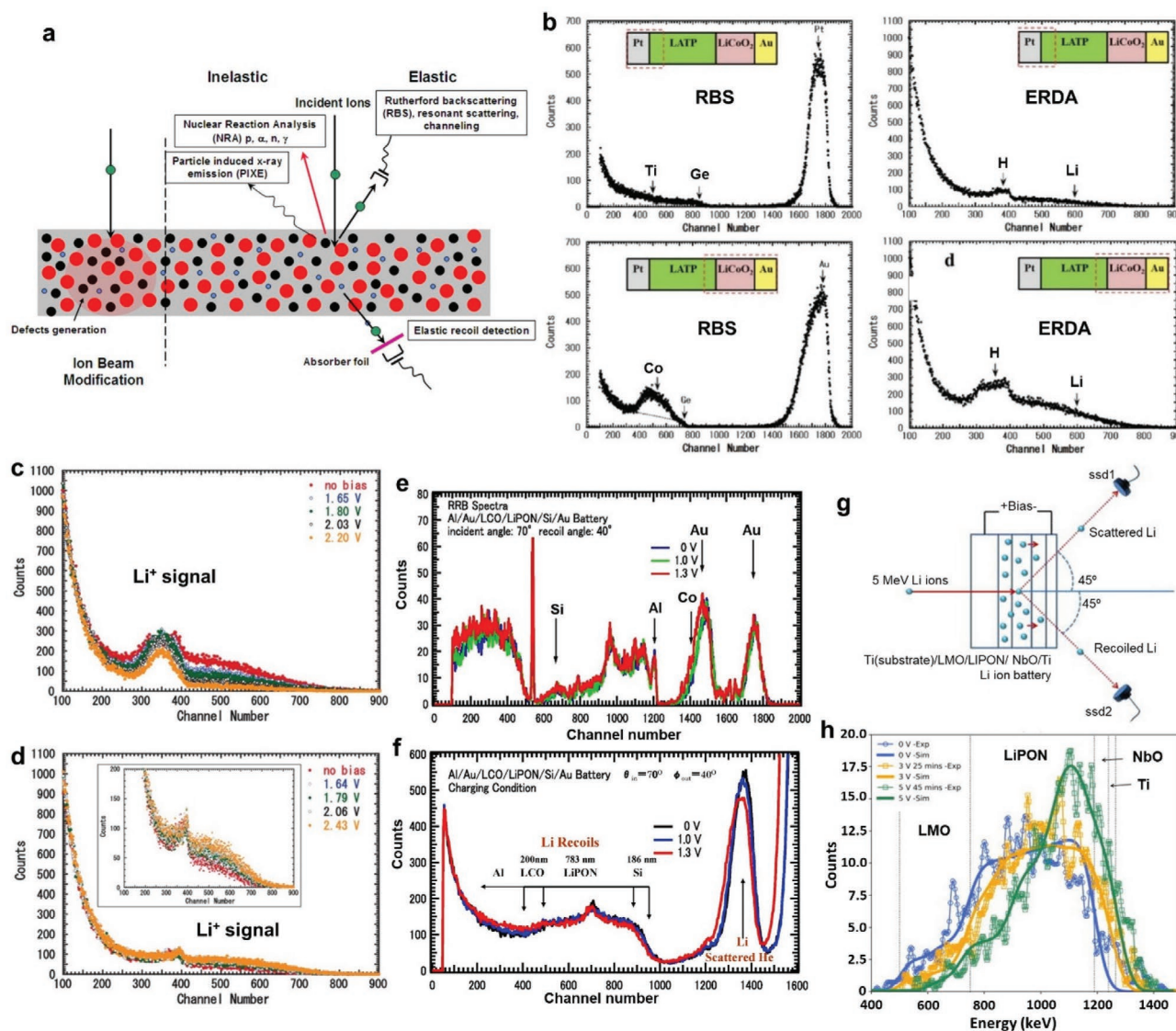
Figure 18. Schematic illustration of the IBA techniques a). RBS and ERDA depth profiles of an as-prepared Pt/Li-Al-Ge-Ti-P-O/LiCoO 2 /Au battery b). The battery was flipped during the measurement to gain access from both sides. In situ ERDA spectra collected from the Li-Al-Ge-Ti-P-O/LiCoO 2 /Au side c) and from the Pt/Li-Al-Ge-Ti-P-O side d). RBS e), and ERDA f) spectra of a thin film Al/Au/LiCoO 2 /LiPON/Si/Au battery at different SoC measured by 5.4 MeV He 2+ . Schematics of the co-incidence ERDA experiment using 5 MeV 7 Li-ions on a thin-film battery g). Simulated and experimental ERDA spectra of the Ti/NbO/LiPON/LiMn 2 O 4 /Ti ASSB at different SoC h). a) Reproduced with permission. [247] Copyright 2008, Kin Man Yu. b-d) Reproduced with permission. [249] Copyright 2019, Wiley-VCH. e,f) Reproduced with permission. [250] Copyright 2018, Elsevier. g,h) Reproduced with permission. [251] Copyright 2020, AIP Publishing.
