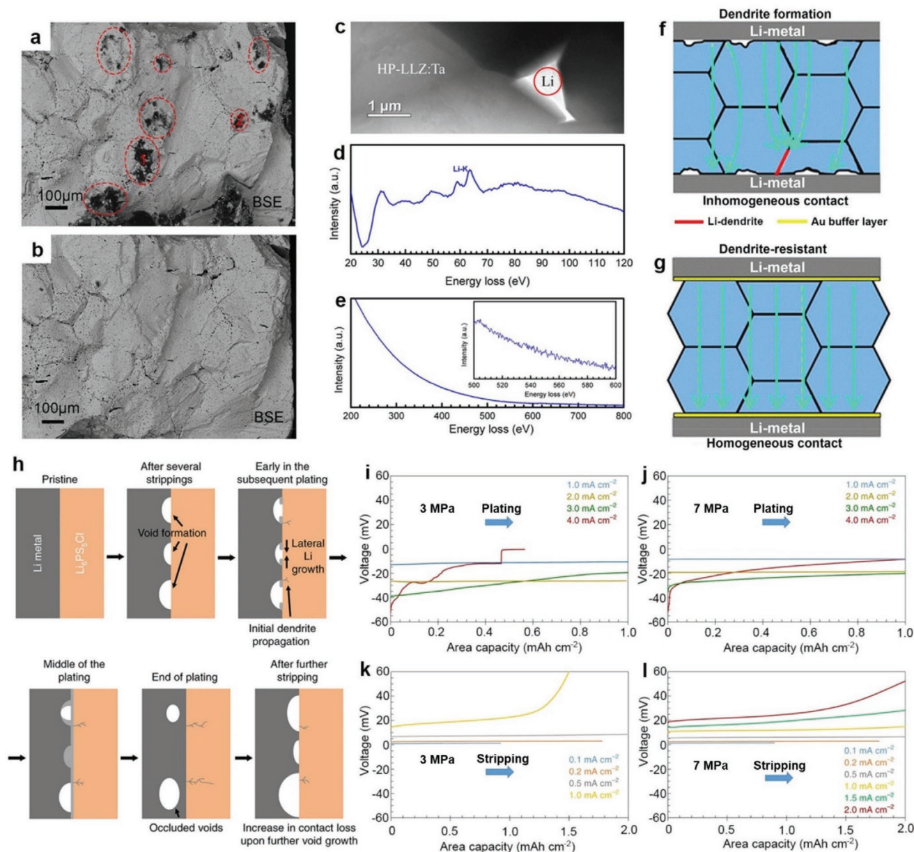
Figure 8. Cross-sectional SEM images of a short-circuited Li 6.75 La 3 Zr 1.75 Ta 0.25 O 12 pellet before a) and after ethanol rinsing b). TEM image c) and EELS d, e) of a Li 7 La 3 Zr 2 O 12 pellet from a shorted battery. Schematic illustration of the current flow pathways at a rough f) and smooth interface g). Evolution scheme of a Li/Li 6 PS 5 Cl interface when cycled at an applied current density above the critical current density h). Voltage-charge plots for three-electrode Li/Li 6 PS 5 Cl batteries at different indicated pressures and current densities i-l). a, b) Reproduced with permission. [97] Copyright 2015, Elsevier. c-g) Reproduced with permission. [66] Copyright 2016, American Chemical Society. h-l) Reproduced with permission. [67] Copyright 2019, Springer-Nature.
