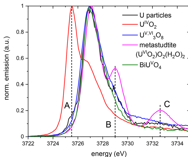
urement. Right: Normalised \text{U M}_4 HR-XANES spectra of U microparticles deposited on a glass disc (black solid line) in comparison to U reference compounds. The vertical dashed line A indicates the WL position obtained for \text{UO}_2 (3725.5 eV), lines B and C mark spectral features characteristic for uranyl-type species as in schoepite or metastudtite. The sample was stored for ten months under laboratory atmosphere before measurement
