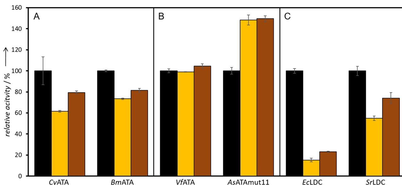
Figure 4. Relative activities of the CvATA (0.5 mg/mL), BmATA (0.1 mg/mL), VfATA (0.05 mg/mL) and AsATAmut11 (1 mg/mL) for the formation of acetophenone (6) and of the EcLDC (0.05 mg/mL) and SrLDC (0.025 mg/mL) for the formation of cadaverine (9) using dark conditions (■), normal light conditions with a light intensity of \sim 0.25 \text{ mW/cm}^2 (■) and mixed conditions (■), grouped in three categories (A–C) depending on the level of inactivation. ATA reactions contained 30 mM ( rac )- \alpha -MBA (4), 60 mM pyruvate (5) and 0.1 mM PLP in 100 mM HEPES buffer (pH 7.5) at 20 °C and 600 rpm. LDC reactions were performed using 10 mM L-lysine (8), 0.1 mM 4-nitrophenol and 0.1 mM PLP in 25 mM HEPES buffer (pH 6.0) at 20 °C. The error bars represent the standard deviation of technical triplicates.
