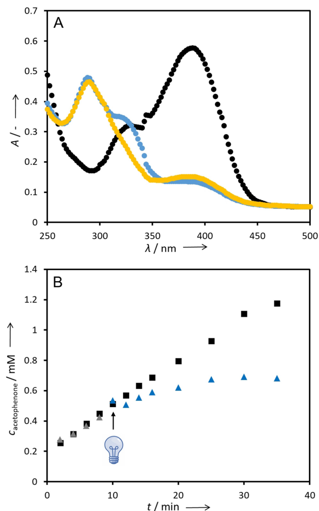
Figure 2. (A) Spectrophotometric analysis of 0.1 mM PLP solutions in 100 mM HEPES buffer (pH 7.5) after 60 min of incubation in the dark (●), in normal light conditions with a light intensity of \sim 0.25 \text{ mW/cm}^2 (●) and with blue light illumination of \sim 60 \text{ mW/cm}^2 using a single LED (●). Samples were incubated at 22^\circ\text{C} and 600 rpm. (B) Acetophenone (6) formation by 0.03 mg/mL purified CvATA over the course of 35 min in the dark (■) and with blue light illumination of \sim 12 \text{ mW/cm}^2 using LED strips (60 LEDs; ▲). Before blue light illumination, the enzymatic reaction was initiated in the dark for 10 min (▲), including 30 mM ( rac )- \alpha -MBA (4), 60 mM pyruvate (5) and 0.1 mM PLP in 100 mM HEPES buffer (pH 7.5) at 22^\circ\text{C} and 600 rpm.
