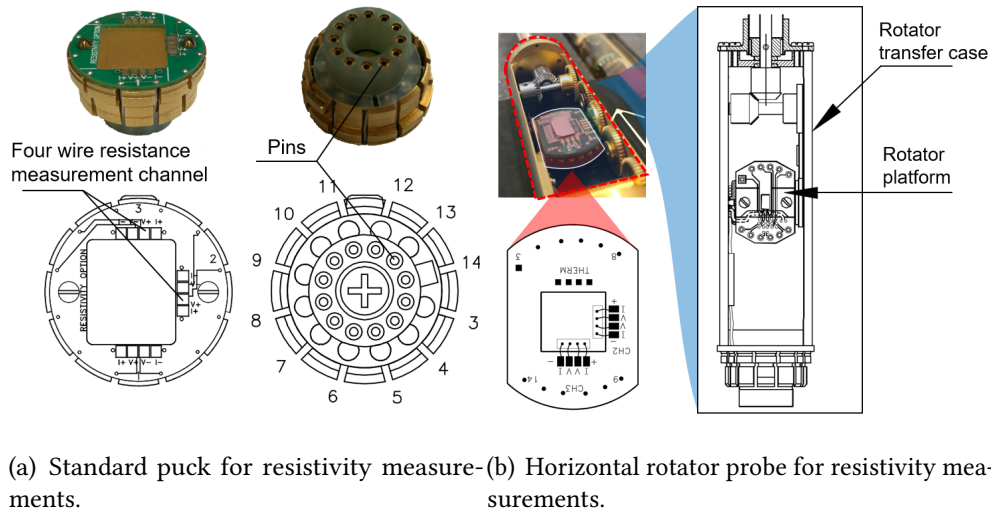
Figure 3.12: Pictures and schematic sketches of a standard PPMS puck (a) and a horizontal rotator probe (b) for resistivity measurements. There are three channels available to perform four-wire resistance measurements and 12 pins to connect to the sample chamber on a standard resistivity puck(a). There is a rotatable platform with a sample holder board in a horizontal rotator probe(b) [27]. The sample holder board has two channels for four-wire resistance measurements.
