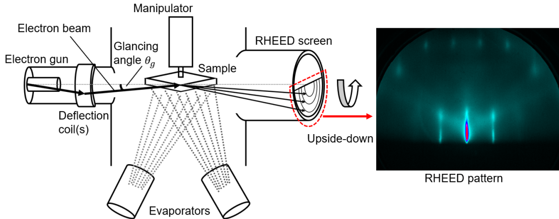
Figure 3.3: Schematic setup of a RHEED. A high energy electron beam hits the sample with a small glancing angle \theta_g . Electrons can interfere constructively to form a diffraction pattern on the RHEED screen to enable the in-situ characterization during the sample growth.
