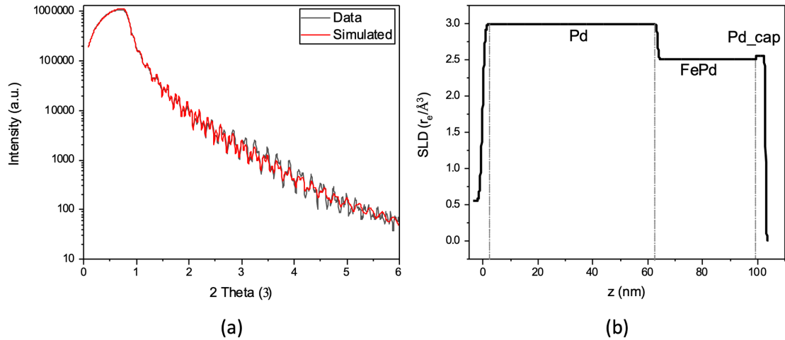
Figure 4.9: (a) X-ray reflectometry measurement of the sample 0663. The XRR data could only be simulated roughly. (b) The SLD as a function of the height above the substrate.
