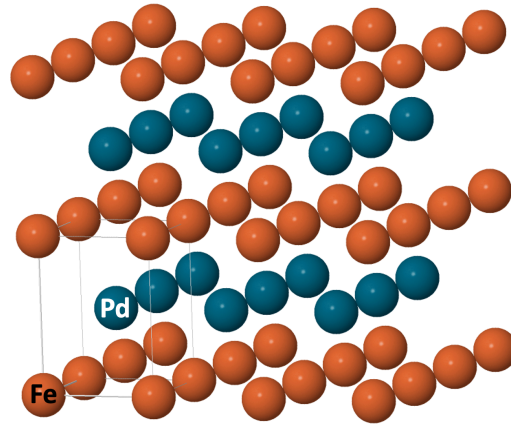
Figure 2.4: Alternative atomic stack of FePd with L1_0 -ordered structure [11]. The 3D-model of the lattice structure is exported from [12].
