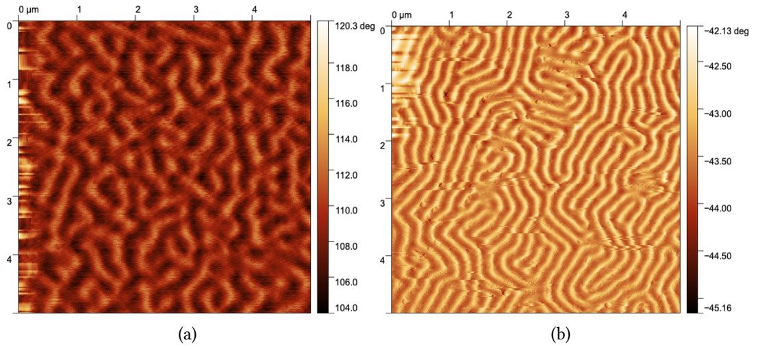
Figure 4.29: 5×5 μm MFM images of high PMA (a) and low PMA (b) after out-of-plane demagnetization. The domain wall density of high PMA sample is much lower than that of low PMA sample.
