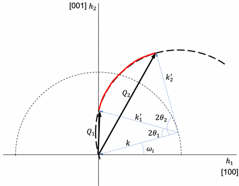
(b) The calculation of the reciprocal data from the WAXS data. \omega_i is the rotation angle of the sample, k is the incident wave vector, k'_1 and k'_2 are diffracted wave vectors at 2\theta_1 and 2\theta_2 , Q_1 and Q_2 are the scattering vectors at 2\theta_1 and 2\theta_2 .
