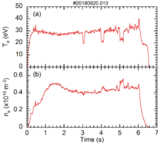
Figure 8. Electron temperature (a) and density (b) measured by Langmuir probes as shown in Fig.2. \text{CH}_4 is injected at 3 s, 4 s and 5 s with a injection length 100 ms, 150 ms and 200 ms.
