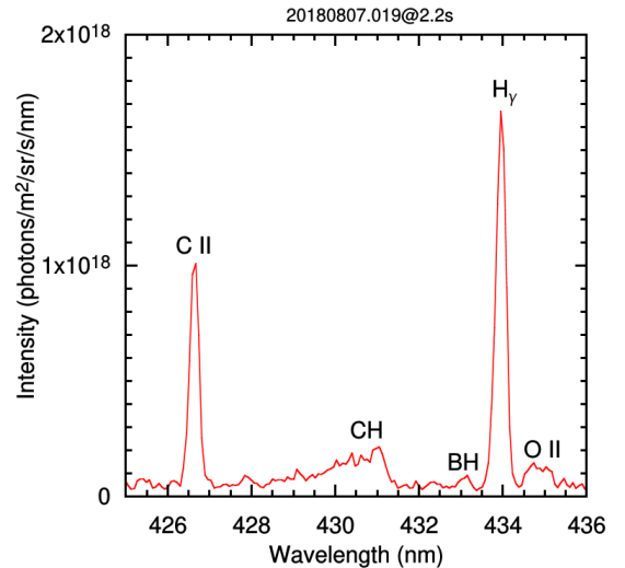
Figure 9. Typical spectrum of CH Gerö band measured in a hydrogen discharge with injecting power P_{\text{ECRH}} = 2.3\text{MW} and line integrated density is n_e = 7.4e19\text{ m}^{-2} .
