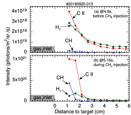
Figure 7. CH , H\gamma and C II penetration depth in radial direction before (a) and during (b) CH_4 injection measured by SP2750 spectrometer (horizontal LOS).
