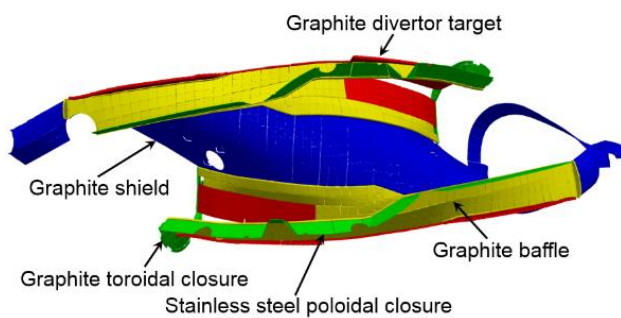
Figure 1. One fifth of the circumference of W7-X with the inertially cooled plasma-facing components installed in OP1.2a.
