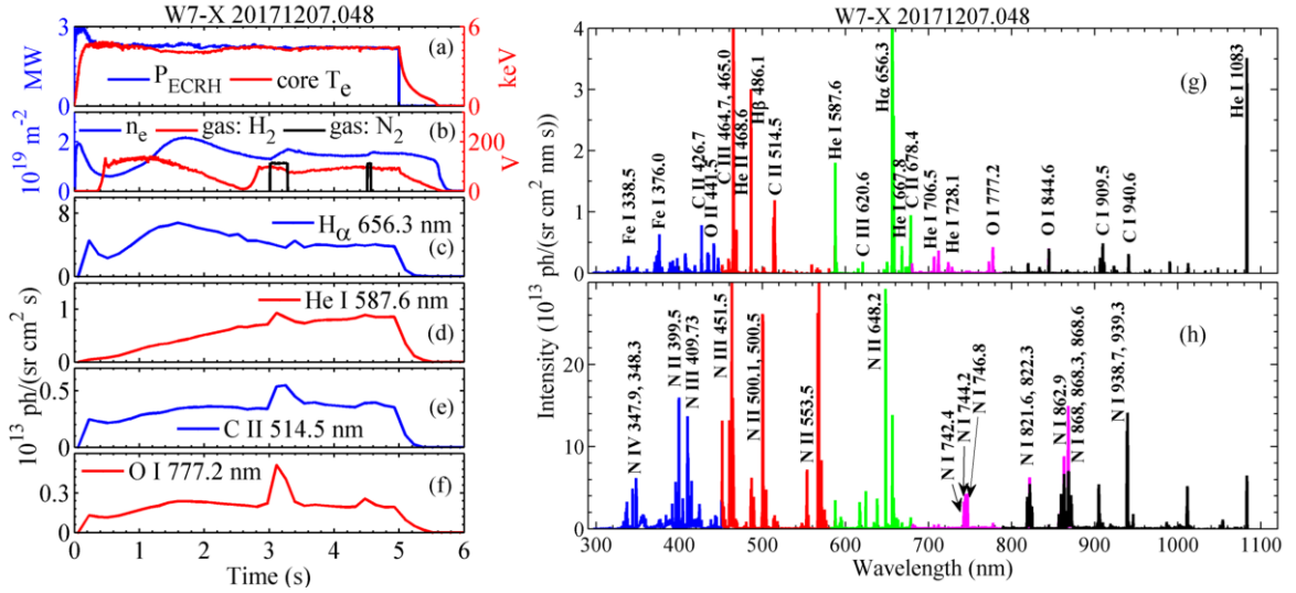
Figure 3. Overview of a typical hydrogen discharge with nitrogen seeding through the divertor gas inlet. The time traces in the left figure from top to bottom are (a) the ECRH heating power ( P_{\text{ECRH}} ), and the core electron temperature (core T_e ), (b) the line-integrated electron density ( n_e ), and the valve voltage of main gas fuelling system ( \text{H}_2 ) and divertor gas inlet ( \text{N}_2 ), (c) the \text{H}_\alpha photon flux, (d) the He I photon flux, (e) the C II photon flux and (f) the O I photon flux. The spectra before and during nitrogen seeding are plotted in the right figure (g) and (h) with spectral lines of H, He, C, O, Fe and N identified and labeled.
