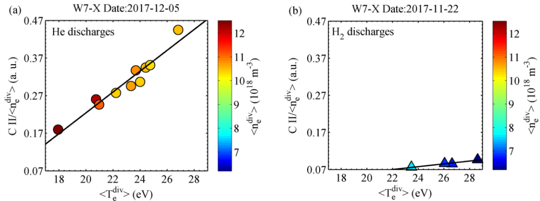
Figure 13. Parametric dependence of the normalized particle flux C\ II/\langle n_e^{\text{div}} \rangle on divertor temperature and density for (a) a series of continuous helium discharges and (b) a series of continuous hydrogen discharges. The ranges of horizontal and vertical axes and the color bar range for divertor density are the same for the frames (a) and (b). The C\ II/\langle n_e^{\text{div}} \rangle increases with increasing divertor T_e .
