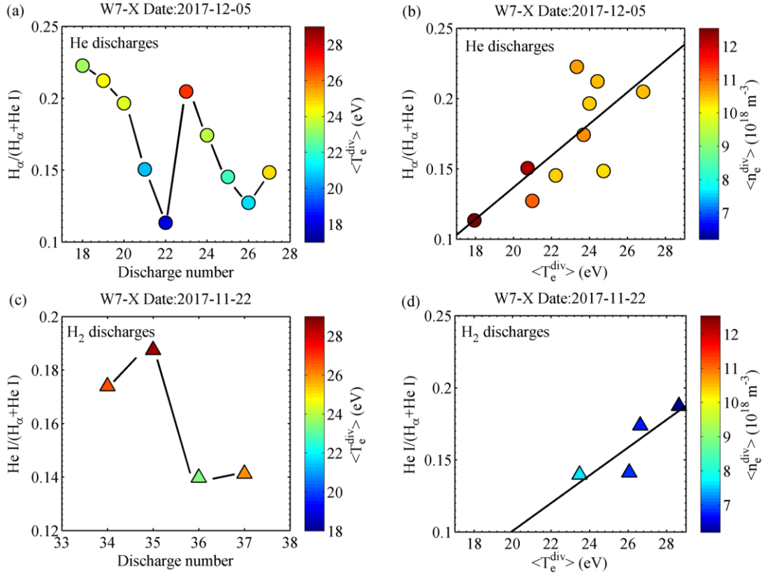
Figure 11. The particle flux ratio \text{H}_\alpha/(\text{H}_\alpha + \text{He I}) over a series of continuous helium discharges (a) and the dependence of the \text{H}_\alpha/(\text{H}_\alpha + \text{He I}) ratio on the divertor temperature and density (b). The particle flux ratio \text{He I}/(\text{H}_\alpha + \text{He I}) over a series of continuous hydrogen discharges (c) and the dependence of the \text{He I}/(\text{H}_\alpha + \text{He I}) ratio on the divertor temperature and density (d).
