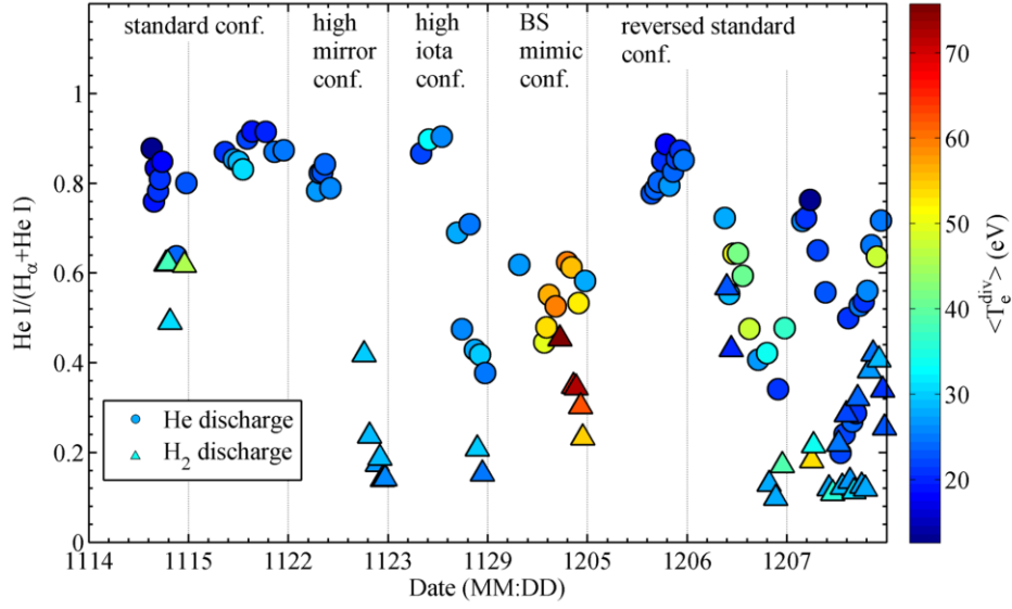
Figure 10. The evolution of particle flux ratio \text{He I}/(\text{H}_\alpha + \text{He I}) in helium and hydrogen discharges as a function of time from November 14 th to December 7 th .
