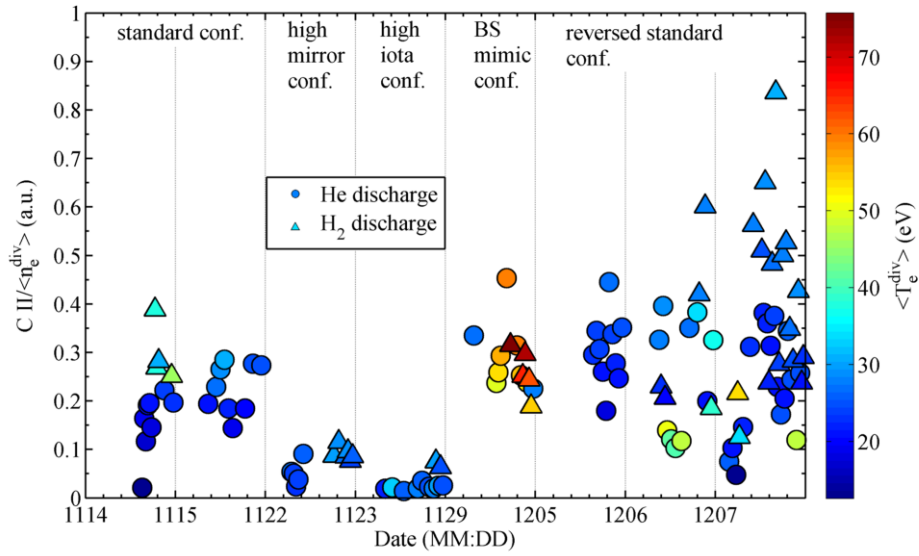
Figure 12. The evolution of the normalized particle flux C\ II/\langle n_e^{\text{div}} \rangle in helium and hydrogen discharges as a function of time from November 14 th to December 7 th .
