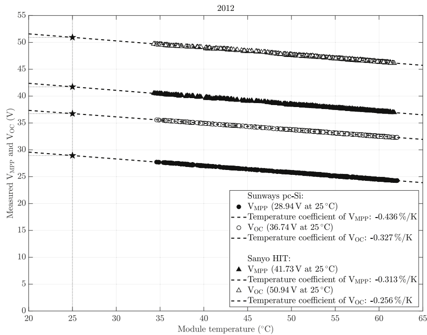
Fig. 9. Linear regression of V_{OC} and V_{MPP} measurements at an irradiance interval of 1000 \pm 10 \text{ W/m}^2 with respect to the module temperature measurements of both module technologies in 2012.
