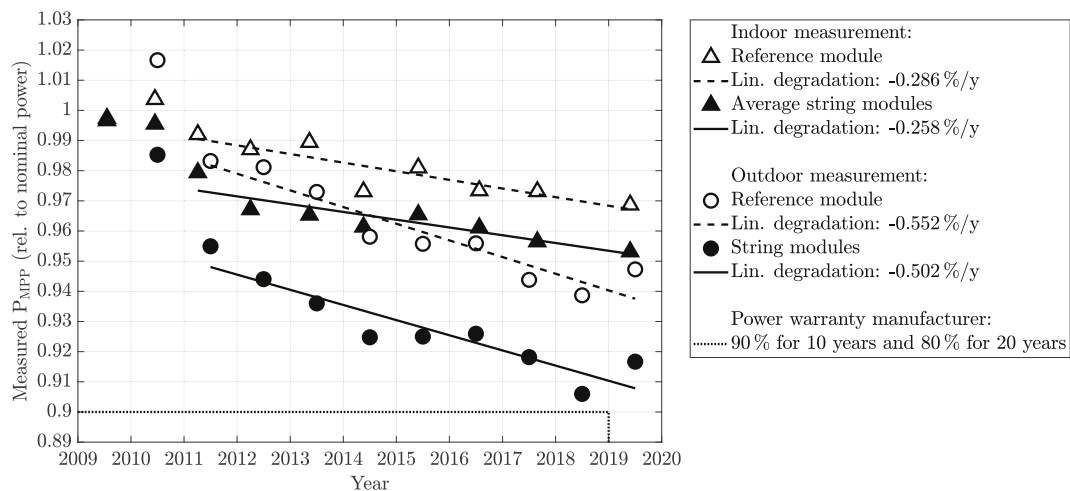
Fig. 5. Measured P_{MPP} relative to nominal power of the HIT modules determined by the indoor and outdoor methodology and their corresponding degradation rates.
