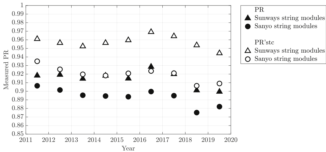
Fig. 8. The PR and PR STC are calculated for the multi c-Si and HIT string modules.
