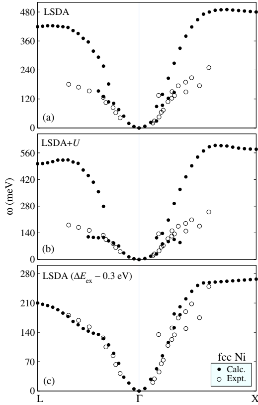
FIG. 8. Spin-wave dispersion for fcc Ni along high-symmetry lines (L-Γ-X) in the Brillouin zone within (a) LSDA, (b) LSDA + U , and (c) LSDA with a reduced exchange splitting. The experimental dispersion is taken from Refs. 70 and 86.
