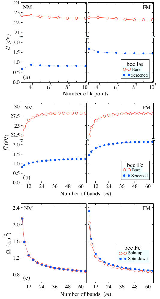
FIG. 3. (Color online) Convergence of the average on-site matrix elements of the bare and screened Coulomb interactions between the 3d orbitals as a function of (a) the number of \mathbf{k} points and (b) the number of bands used in the construction of the MLWF basis for the NM and FM states of bcc Fe. (c) The same as (b) for the average spread of the 3d orbitals.
