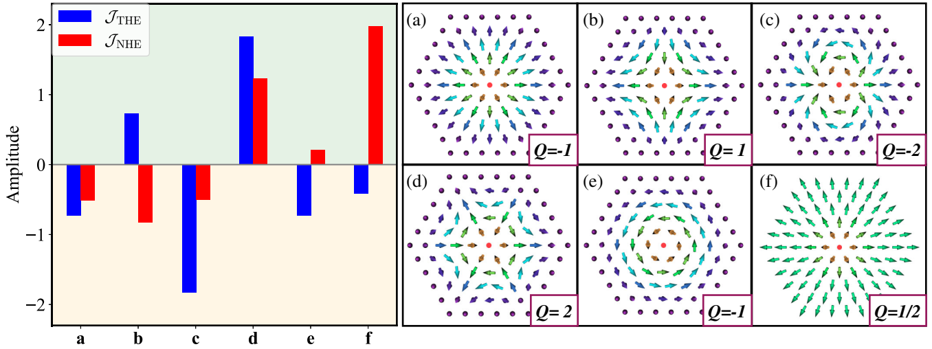
FIG. 2. The chart in the left panel describes the size of the topological (blue) and noncollinear (red) Hall current for six topological spin textures calculated for Rashba-type SOC with spin-orbit strength of \mathcal{R} = 25\% . The latter are shown in the right panel: (a) Néel-type skyrmion, (b) anti-skyrmion, (c) bi-skyrmion, (d) anti-bi-skyrmion, (e) Bloch-type skyrmion, (f) meron. We consider clusters containing 91 magnetic sites with a nearest neighbor distance of d = 3 \text{ \AA} . Smearing \Gamma = 0.2 \text{ eV} is used in the vicinity of the Fermi energy to account for eventual temperature or disorder effects.
