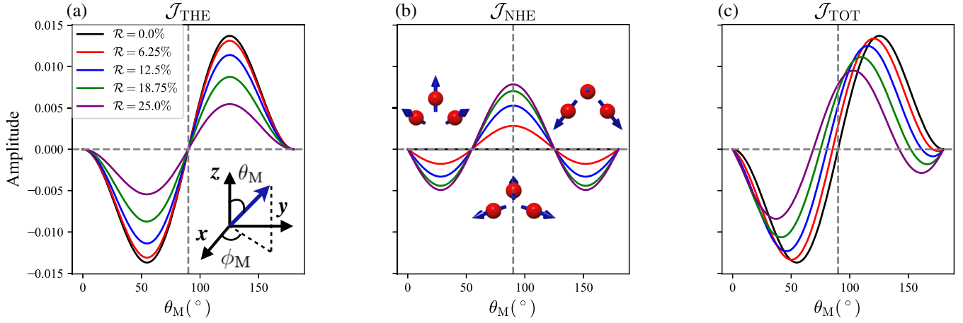
FIG. 1. Evolution of the scattered current for a magnetic trimer in an equilateral geometry as a function of the opening angle \theta_M of the magnetic moments and of the spin-orbit strength \mathcal{R} . (a) The THE contribution to the current determined by the scalar spin chirality. (b) NHE current originating from relativistic effects, its nontrivial angular dependence is given in Eq. (2). (c) Total Hall current emerging from three spin processes, which present a nonsymmetric dependence for \theta_M \rightarrow \pi - \theta_M .
