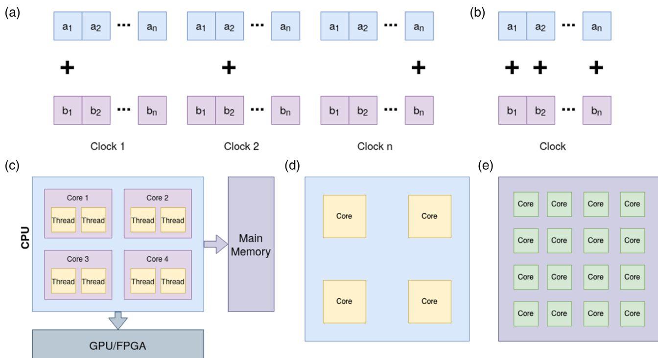
FIGURE 1 Addition with scalar operations (a) and with SIMD (b). Schematic of a computer system with multi-core CPU and with an accelerator (c). Schematic of a CPU (d) and a GPU (e) architecture
