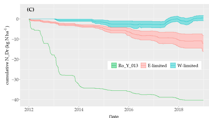
Figure 3. For the period between 2012 and 2018 in Selhausen, the water-limited site (W-limited) and Rollesbroich, the energy-limited site (E-limited), (A) daily precipitation (Prec) and actual evapotranspiration (ETa), (B) cumulative net drainage (Dr), (C) cumulative net leached nitrogen (N_Dr). For (B) and (C), the colored areas represent the standard deviation to the mean value of each study site. For (C), because E-limited Ro_Y_013 behaved differently compared with the other E-limited lysimeters, its dataset is presented separately.
