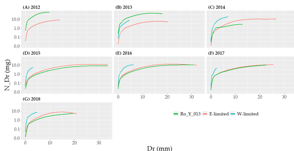
Figure 6. Interpolated relations of nitrogen mass in drainage ( \text{N}_\text{Dr} ) versus the amount of drainage ( \text{Dr} ) from the Rollesbroich lysimeters obtained from data pairs of the 14-days sampling periods between 2012 and 2018, for the lysimeters in Selhausen, the water-limited site (W-limited), the lysimeter Ro_Y_013 and the other lysimeters in Rollesbroich, the energy-limited site (E-limited). Because E-limited Ro_Y_013 behaved differently compared with the other E-limited lysimeters, its dataset is presented separately. The interpolation was done using a Locally Estimated Scatterplot Smoothing function with a span of 0.75. No observations of \text{N}_\text{Dr} were available for Selhausen in 2012.
