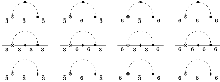
Figure 2. Different combinations of the spin-1/2 anti-triplet and sextet charmed baryons contributing to F_3(q^2) .
