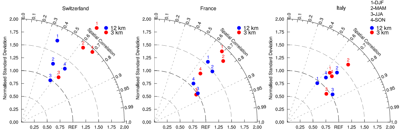
Fig. 9 Spatial Taylor diagrams exploring the multi-model mean performance with respect to the spatial variability of mean seasonal daily precipitation over the three regions—Switzerland, France, and Italy. The diagrams combine the spatial correlation ( \cos(\text{azimuth angle}) )
