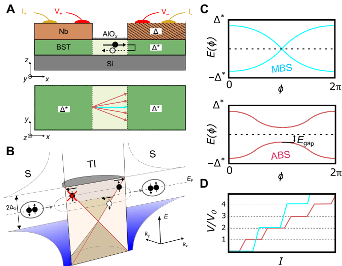
Fig. 1. Schematic representation of the BST thin-film Josephson junctions. (A) The Nb electrodes described by the order parameter \Delta induce a proximity coupled order parameter of size \Delta^* \leq \Delta within the BST thin film underneath. Within the nonproximitized regions of the BST thin film, a supercurrent will flow, which is carried by MBSs (turquoise) and ABSs (magenta). (B) A supercurrent of charge 2e is transferred across the TI weak link by coherent electron-hole bound states (dotted line) that are based on the Andreev and reverse Andreev reflection process at the TI/S and S/TI interface, respectively. For perpendicular incident modes [turquoise arrow in (A)], normal reflections at the TI/S interface are suppressed due to orthogonality of both electronic states involved. The resulting bound states are gapless MBSs. For nonperpendicular modes, the probability of normal reflections is nonzero, establishing ABSs with a finite gap E_{\text{gap}} . (C) The relation of the bound states energy with respect to the superconducting phase difference in between the superconducting electrodes is 2\pi -periodic for ABSs and 4\pi -periodic for MBSs. (D) In Shapiro step experiments, the ABSs result in integer steps of the Shapiro step separation voltage V_0 , while MBSs result in only even integer steps.
