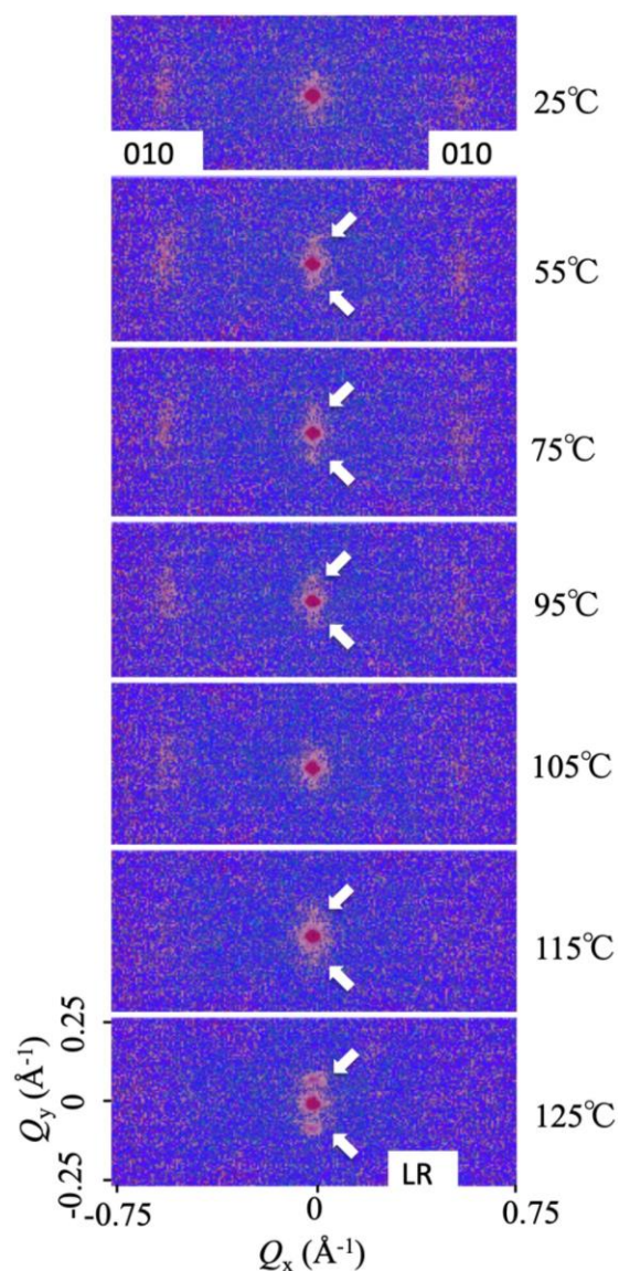
Fig. 3. Temperature dependent SANS profile changes of a one-dimensionally oriented film of sPS/MeBA cocrystal. The Q_x and Q_y directions are parallel to the horizontal and vertical axes. The white arrows indicate the lamellar reflections.
