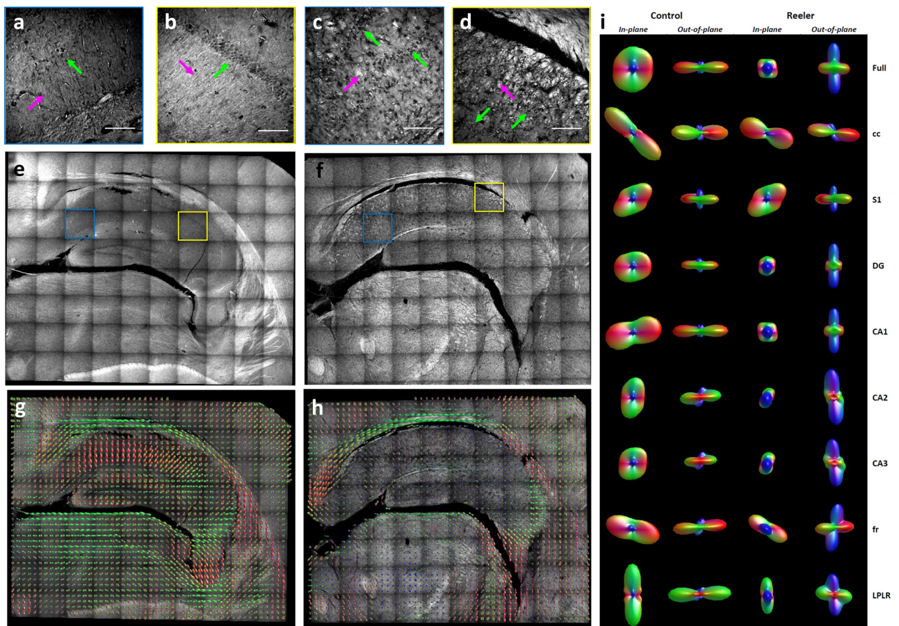
Figure 4. Fibers' orientation in Control and Reeler Hippocampi. ( a–d ) Magnified insets of blue and yellow boxes in e and f , respectively. Green arrows point to neuronal cell bodies, magenta arrows to myelinated fibers. Scale bar = 50 \mu m. ( e, f ) MIP of the mesoscale reconstructions of a control and Reeler mouse hippocampus 60- \mu m-thick coronal section. Scale bar = 1 mm. ( g, h ) Images show the ODF maps obtained from analyzing the full 3D hippocampus reconstruction of the control and the Reeler mouse, sampling 16 vectors for each ODF. ( i ) In-plane and out-of-plane orientation of the single ODF obtained by analyzing all the vectors of the full mosaic reconstructions and each of its ROIs. Acronyms list = cc: Corpus Callosum; S1: Primary Somatosensory Cortex; DG: Dentate Gyrus; CA1, CA2, CA3: field CA1, CA2, CA3 of hippocampus; fr: Fasciculus Retroflexus; LPLR: Lateral Posterior Thalamic Nucleus. Images were prepared using Fiji ( www.fiji.sc/Fiji ) 20 while ODF representations using MRtrix3 ( https://mrtrix.readthedocs.io/en/latest/ ) 26 .
