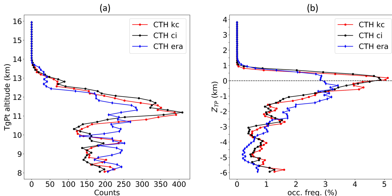
Figure 9. (a) Number of cloud top heights (CTHs) per altitude bin for the extinction method (kc) in red, the CI method (ci) in black and ERA5 (blue). The altitude of the tangent points (TgPt) is the y axis. (b) The same as panel (a) but using as coordinates the distance of the CTHs to the tropopause in km ( Z_{TP} ). The used tropopause is the median tropopause ( TP_{med} ). The three profiles were smoothed with a three points running mean.
