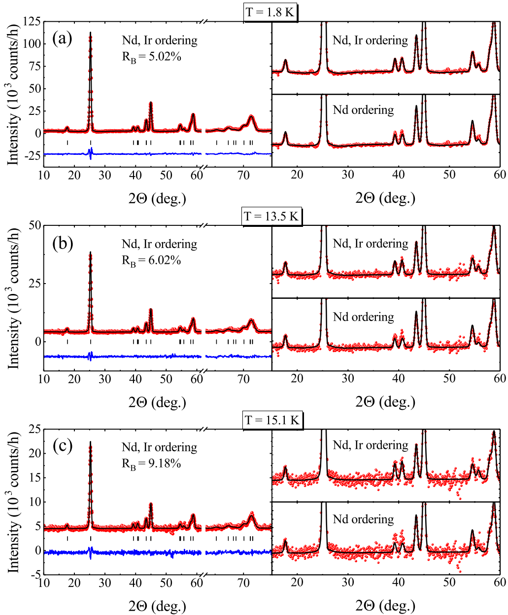
FIG. 5. Rietveld magnetic refinement of the difference pattern at various temperatures for \text{Nd}_2\text{ZnIrO}_6 according to \text{IR } \Gamma_1 + \Gamma_3 . The left panels show the refinement results with perfectly ordered Nd and Ir sublattices, and the right panels highlight an expanded region of low peak intensities, comparing our best model and that with only the Nd sublattice ordering. Red dots: experimental data; black curve: calculated data; vertical bars: magnetic peak position; blue curve: difference between the experimental and calculated data. A small angular range around 2\theta = 62^\circ was excluded from the fits due to contamination from the atomic scattering that did not subtract well.
