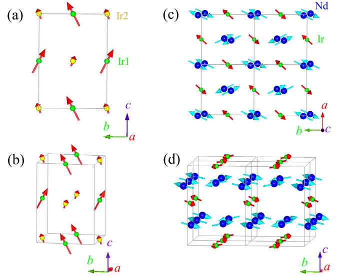
FIG. 5. (Color online) Magnetic structure of (a, b) \text{La}_2\text{ZnIrO}_6 and (c, d) \text{Nd}_2\text{ZnIrO}_6 viewed along different directions. The Ir moments have been enlarged for clarity. Note that the smaller Ir2 moments in (a, b) is visualized taking into account the partial occupation effect.
