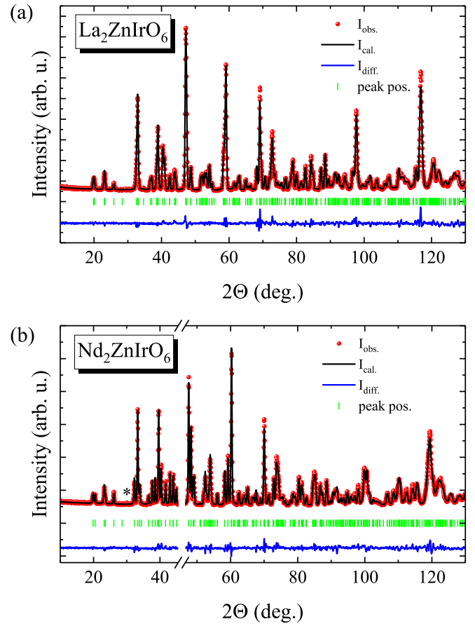
FIG. 1. (Color online) Rietveld refined patterns from R_2\text{ZnIrO}_6 . This high resolution data was collected at room temperature on the D2B diffractometer. The lattice parameters are a = 5.5906(2) Å, b = 5.6871(2) Å, c = 7.9312(2) Å, \beta = 90.00(1)^\circ for R = \text{La} sample and a = 5.4697(2) Å, b = 5.7313(2) Å, c = 7.8058(2) Å, \beta = 89.97(1)^\circ for the R = \text{Nd} sample. A small peak originated from the cryofurnace has been excluded from the refinement in (b), and the asterisk marks the peak originated from the \text{Nd}_2\text{Ir}_2\text{O}_7 phase.
