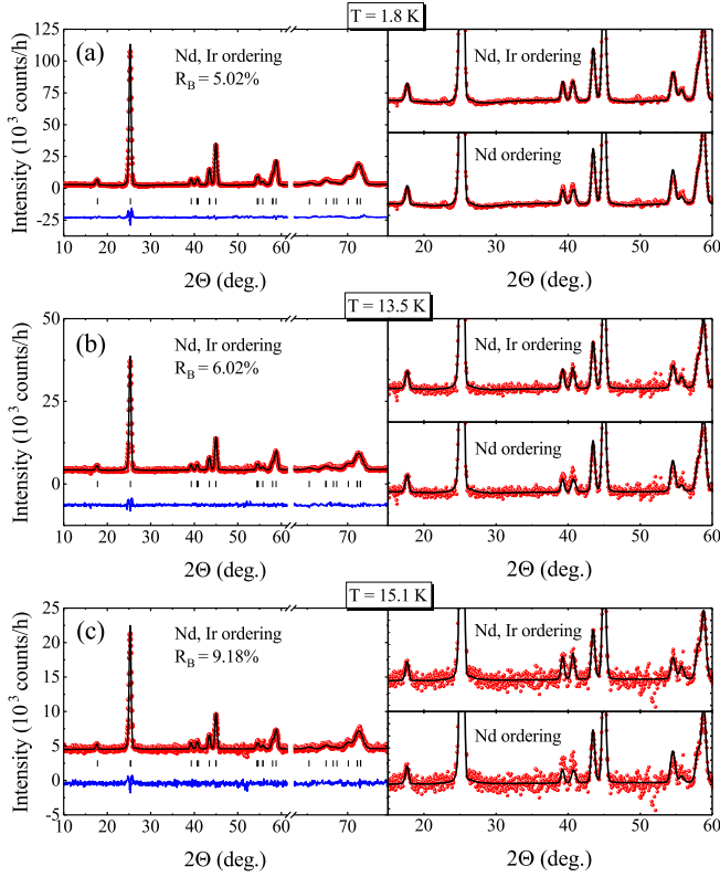
FIG. 4. (Color online) Rietveld magnetic refinement of the difference pattern at various temperatures for \text{Nd}_2\text{ZnIrO}_6 according to IR \Gamma_1 + \Gamma_3 . The left panels show the refinement results with perfectly ordered Nd and Ir sublattices, and the right panels highlights an expanded region of low peak intensities comparing our best model and that with only the Nd sublattice ordering. Red dot: experimental data; Black curve: calculated data; Vertical bars: magnetic peak position; Blue curve: difference between the experimental and calculated data. A small angular range around 2\Theta = 62^\circ was excluded from the fits due to contamination from the atomic scattering that did not subtract well.
