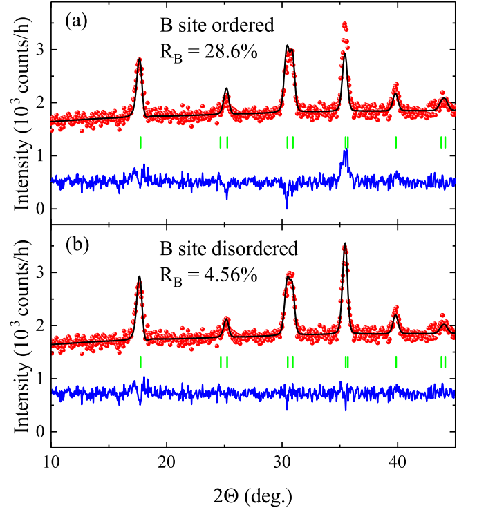
FIG. 3. (Color online) Rietveld refinement of the magnetic diffraction from \text{La}_2\text{ZnIrO}_6 at 1.8 K. A paramagnetic data set, taken at 20 K has been subtracted to remove the scattering from the crystal lattice. The calculated patterns are according to the IR \Gamma_3 with (a) a perfectly ordered B -site model and (b) a B -site disordered model where the best model found 13(4)% site substitution between Zn and Ir ions. Red dot: experimental data; Black curve: calculated data; Vertical bars: magnetic peak position; Blue curve: difference between the experimental and calculated data.
