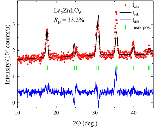
FIG. S1. (Color online) Magnetic structure refinement for \text{La}_2\text{ZnIrO}_6 according to IR \Gamma_1 .
