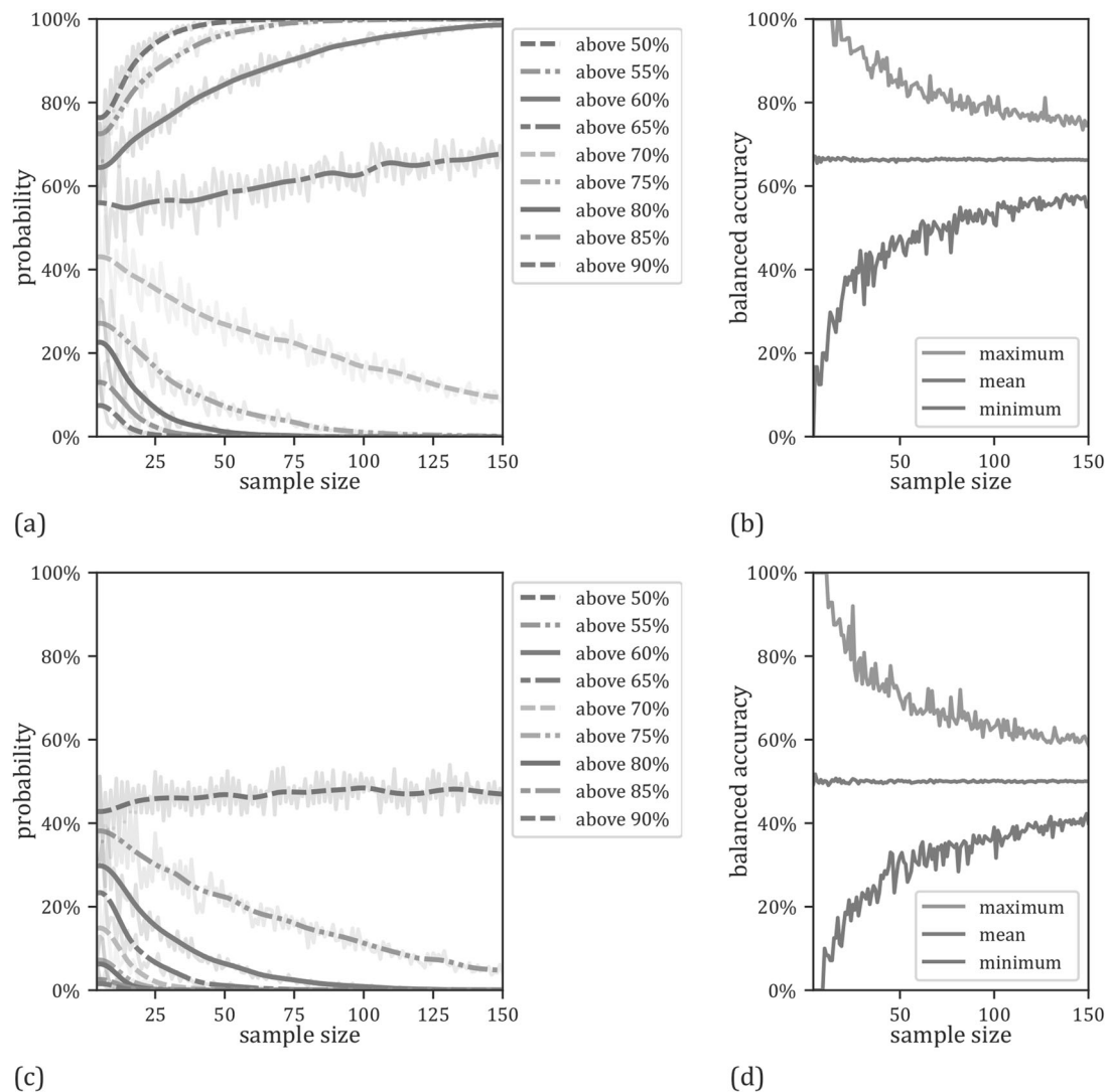
Fig. 4 Results as a function of variable test set sizes with and without a fixed classifier. a Probabilities for linear SVMs to yield an accuracy exceeding a certain threshold as a function of test sample size. b Minimum, maximum and mean results for the linear SVMs as a function of test sample size. c Probabilities for the dummy classifier to get an accuracy above a certain chance level related to the size of the test set size. d Minimum, maximum and mean results for the dummy classifier related to the size of the used sample size for testing.
